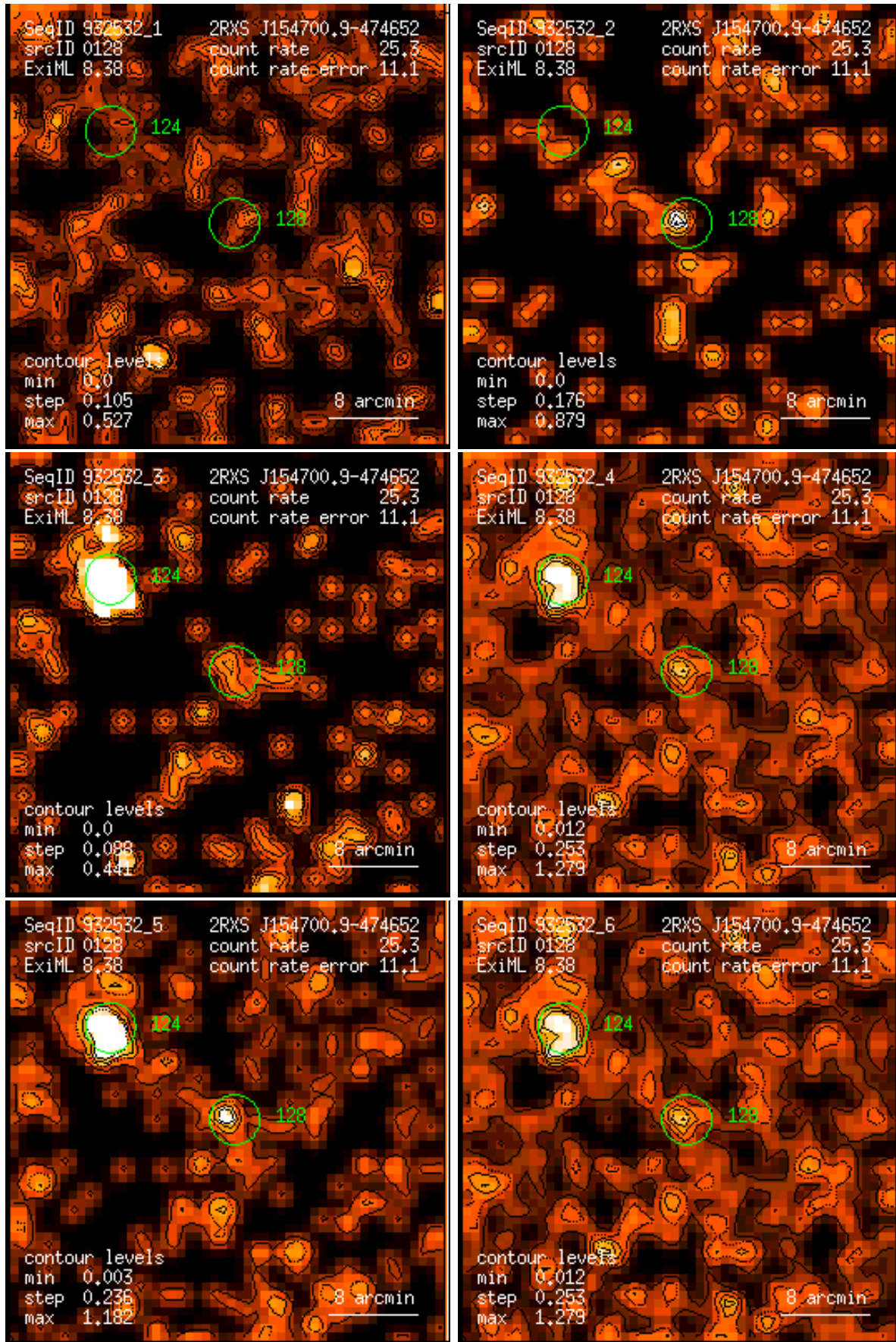
Figure 128: RASS 932532: detection 0128: band rate images, Gaussian filter: (1) PSPC channels 11 – 41, (2) 52 – 90, (3) 91 – 201, (4) 11 – 235, (5) 52 – 201, (6) 11 – 201. Broad band rates in counts/ks. Band rate contour levels in counts/ks/arcmin 2 .
