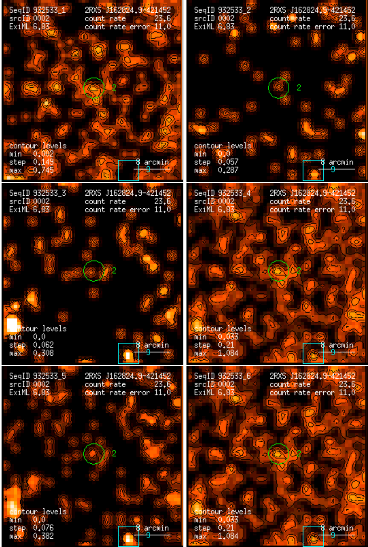
Figure 2: RASS 932533: detection 0002: band rate images, Gaussian filter: (1) PSPC channels 11 – 41, (2) 52 – 90, (3) 91 – 201, (4) 11 – 235, (5) 52 – 201, (6) 11 – 201. Broad band rates in counts/ks. Band rate contour levels in counts/ks/arcmin 2 .
