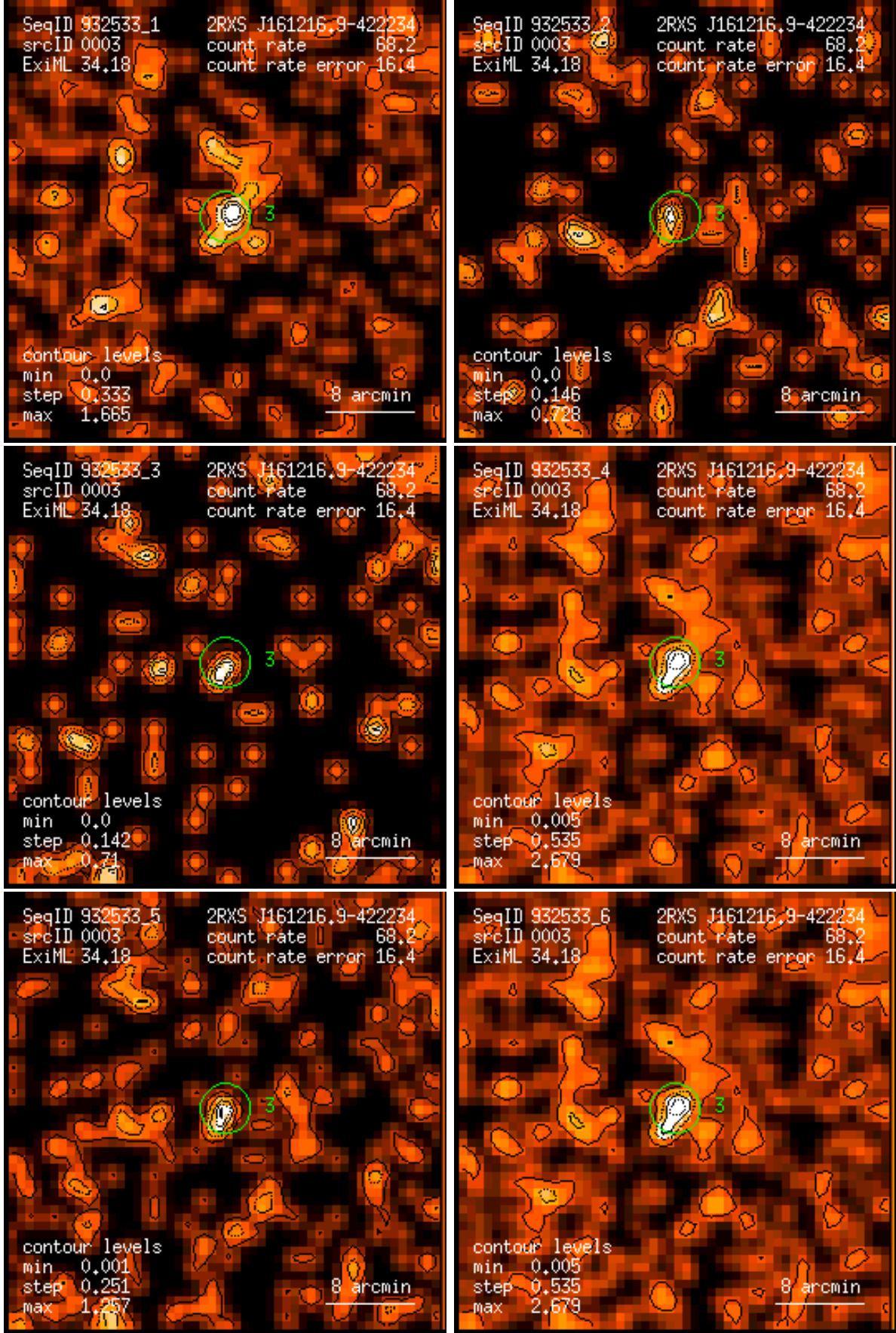
Figure 3: RASS 932533: detection 0003: band rate images, Gaussian filter: (1) PSPC channels 11 – 41, (2) 52 – 90, (3) 91 – 201, (4) 11 – 235, (5) 52 – 201, (6) 11 – 201. Broad band rates in counts/ks. Band rate contour levels in counts/ks/arcmin 2 .
