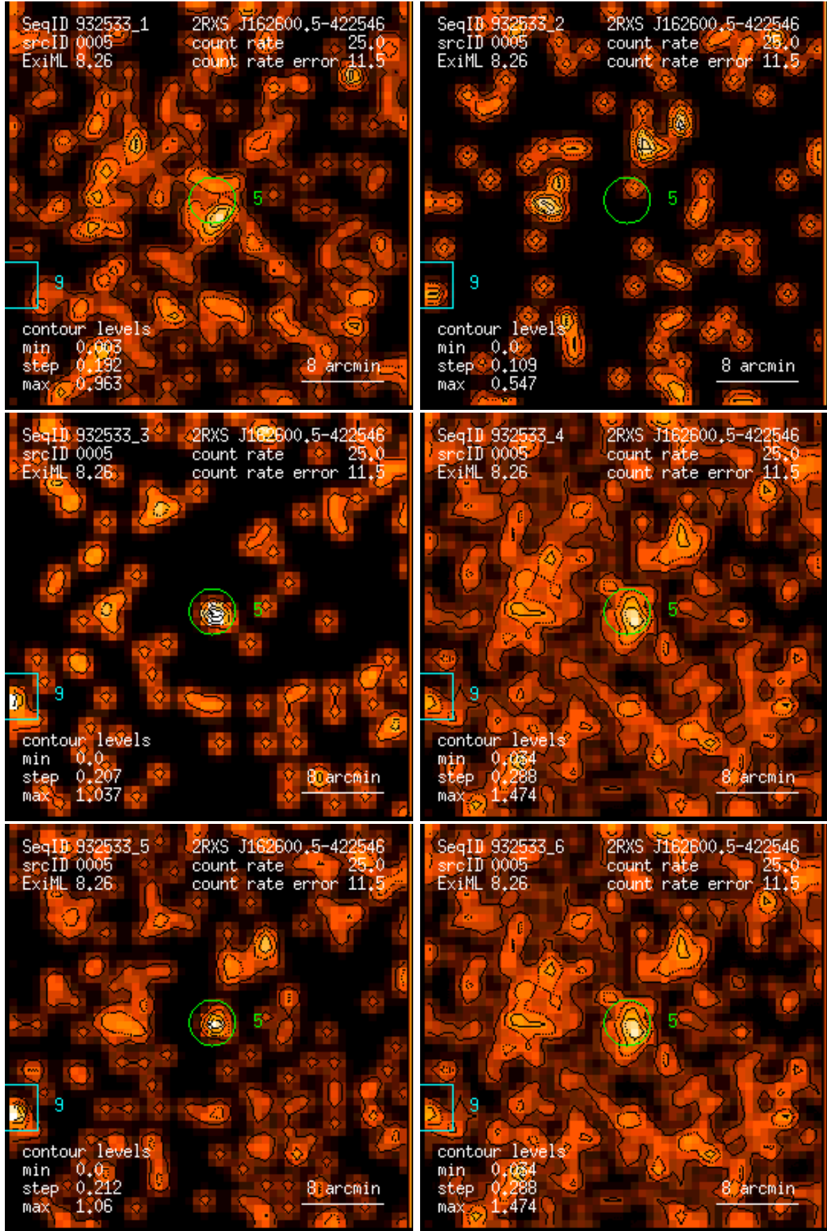
Figure 5: RASS 932533: detection 0005: band rate images, Gaussian filter: (1) PSPC channels 11 – 41, (2) 52 – 90, (3) 91 – 201, (4) 11 – 235, (5) 52 – 201, (6) 11 – 201. Broad band rates in counts/ks. Band rate contour levels in counts/ks/arcmin 2 .
