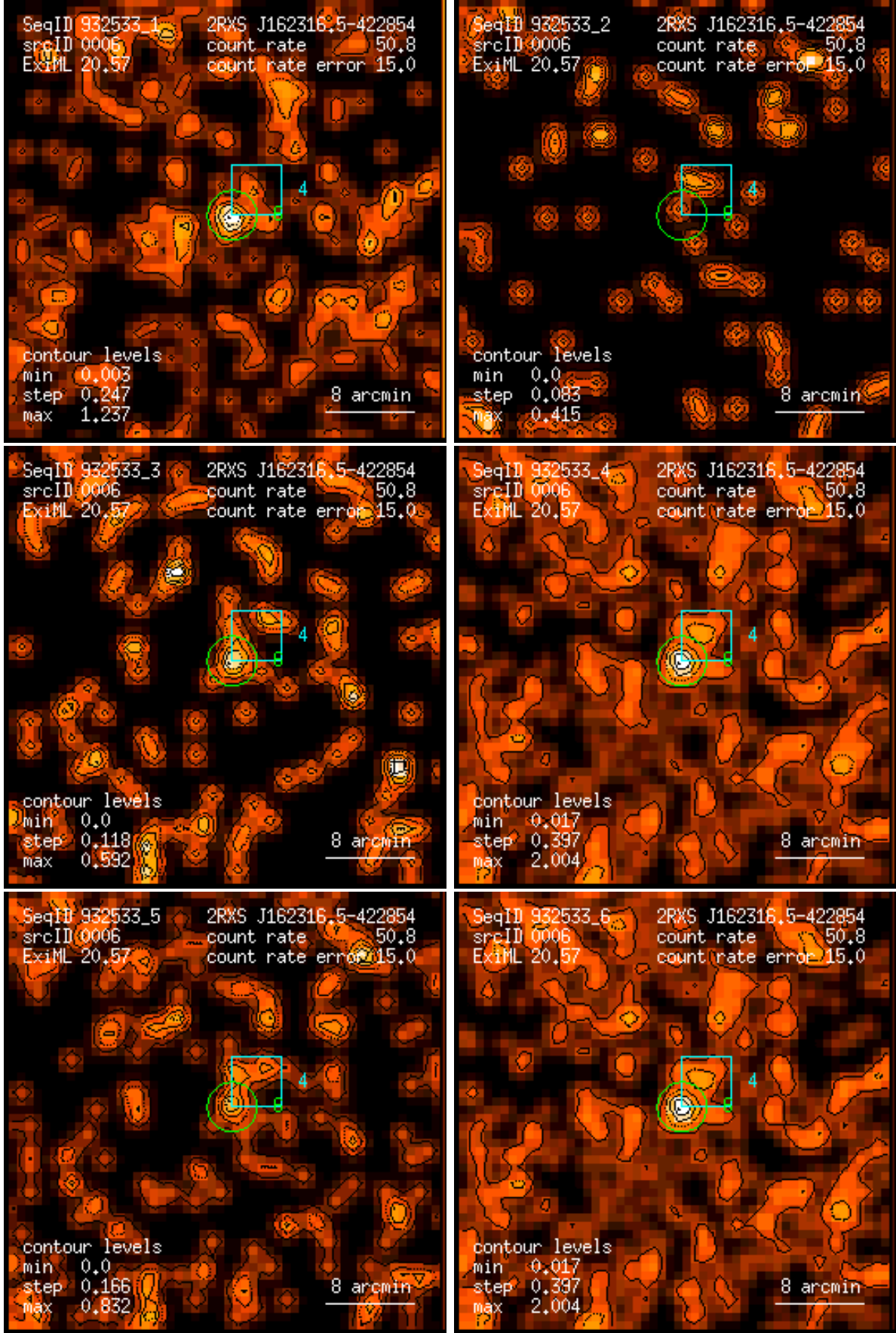
Figure 6: RASS 932533: detection 0006: band rate images, Gaussian filter: (1) PSPC channels 11 – 41, (2) 52 – 90, (3) 91 – 201, (4) 11 – 235, (5) 52 – 201, (6) 11 – 201. Broad band rates in counts/ks. Band rate contour levels in counts/ks/arcmin 2 .
