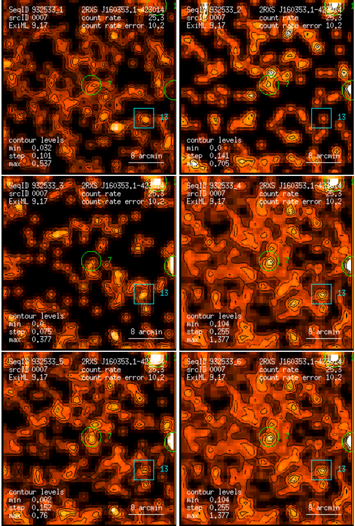
Figure 7: RASS 932533: detection 0007: band rate images, Gaussian filter: (1) PSPC channels 11 – 41, (2) 52 – 90, (3) 91 – 201, (4) 11 – 235, (5) 52 – 201, (6) 11 – 201. Broad band rates in counts/ks. Band rate contour levels in counts/ks/arcmin 2 .
