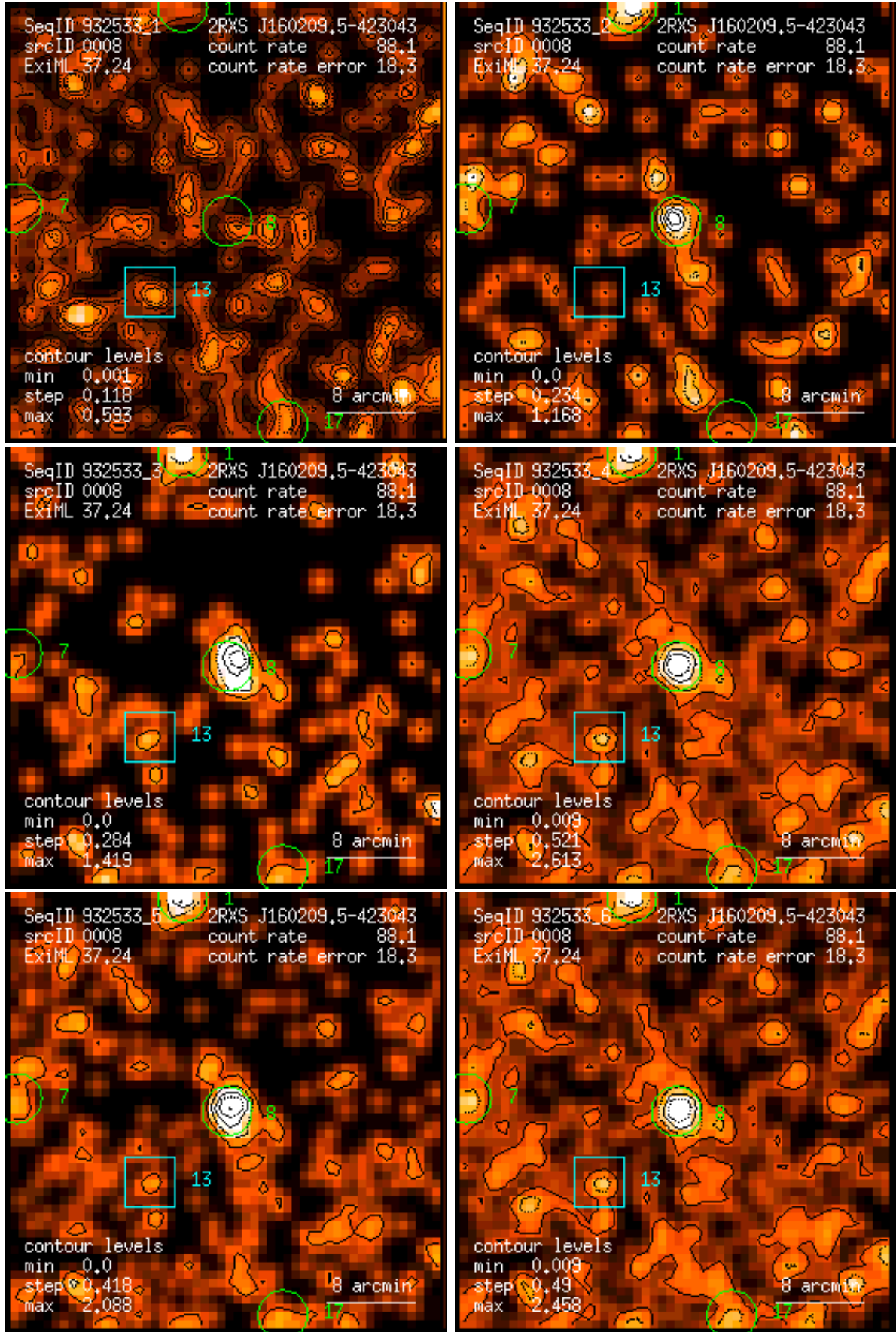
Figure 8: RASS 932533: detection 0008: band rate images, Gaussian filter: (1) PSPC channels 11 – 41, (2) 52 – 90, (3) 91 – 201, (4) 11 – 235, (5) 52 – 201, (6) 11 – 201. Broad band rates in counts/ks. Band rate contour levels in counts/ks/arcmin 2 .
