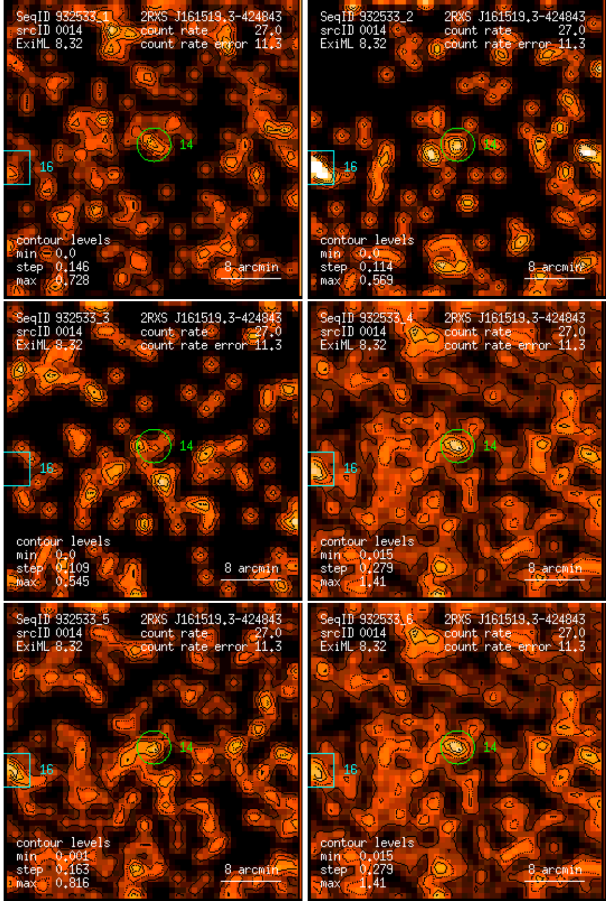
Figure 14: RASS 932533: detection 0014: band rate images, Gaussian filter: (1) PSPC channels 11 – 41, (2) 52 – 90, (3) 91 – 201, (4) 11 – 235, (5) 52 – 201, (6) 11 – 201. Broad band rates in counts/ks. Band rate contour levels in counts/ks/arcmin 2 .
