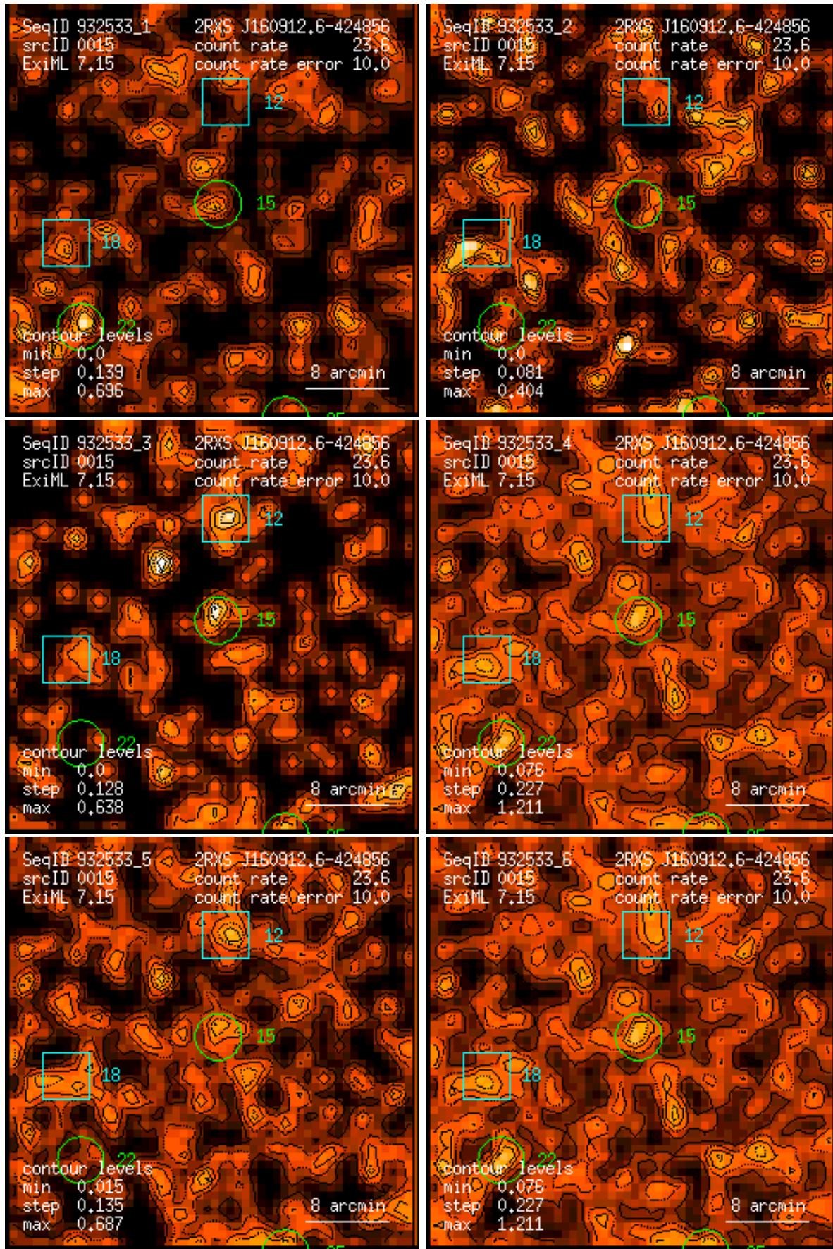
Figure 15: RASS 932533: detection 0015: band rate images, Gaussian filter: (1) PSPC channels 11 – 41, (2) 52 – 90, (3) 91 – 201, (4) 11 – 235, (5) 52 – 201, (6) 11 – 201. Broad band rates in counts/ks. Band rate contour levels in counts/ks/arcmin 2 .
