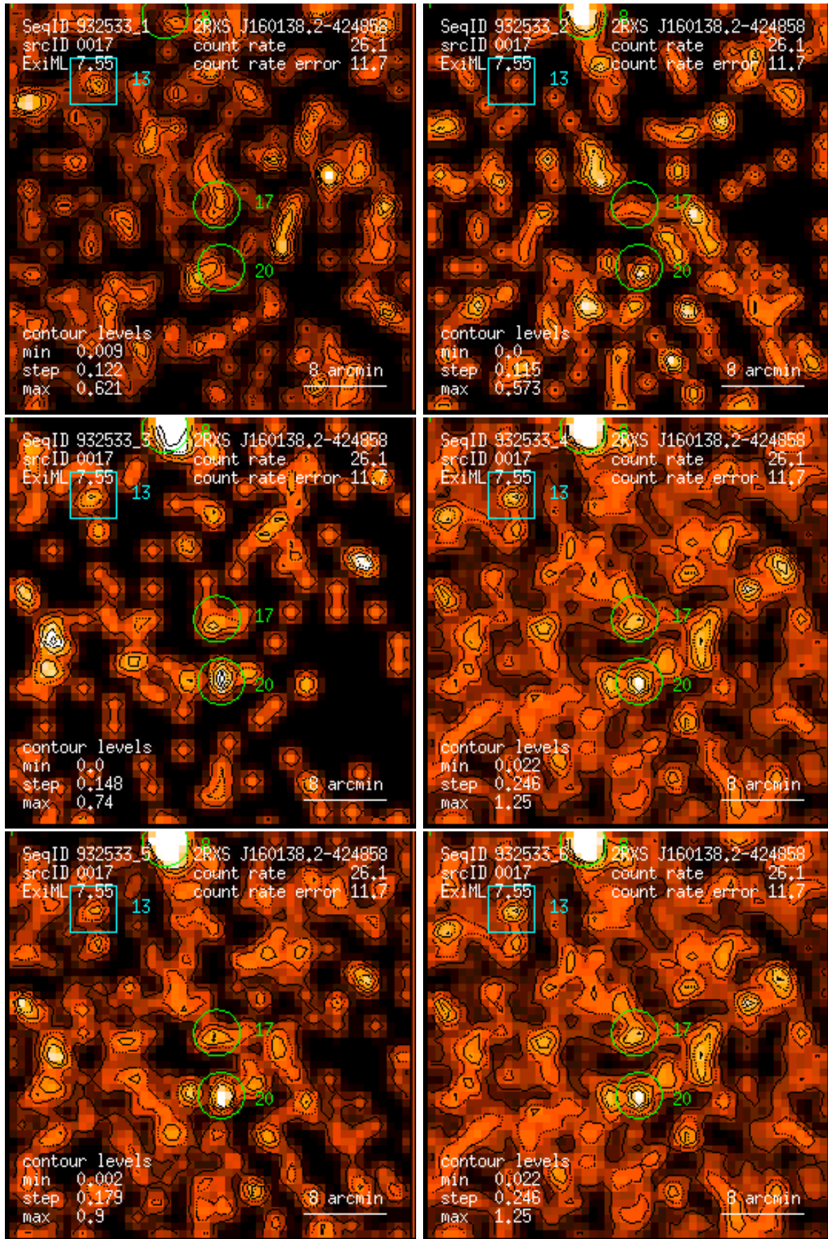
Figure 17: RASS 932533: detection 0017: band rate images, Gaussian filter: (1) PSPC channels 11 – 41, (2) 52 – 90, (3) 91 – 201, (4) 11 – 235, (5) 52 – 201, (6) 11 – 201. Broad band rates in counts/ks. Band rate contour levels in counts/ks/arcmin 2 .
