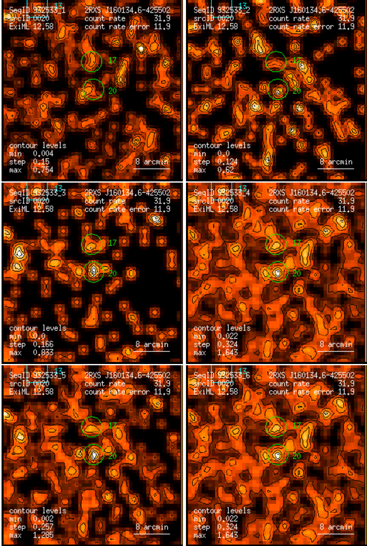
Figure 20: RASS 932533: detection 0020: band rate images, Gaussian filter: (1) PSPC channels 11 – 41, (2) 52 – 90, (3) 91 – 201, (4) 11 – 235, (5) 52 – 201, (6) 11 – 201. Broad band rates in counts/ks. Band rate contour levels in counts/ks/arcmin 2 .
