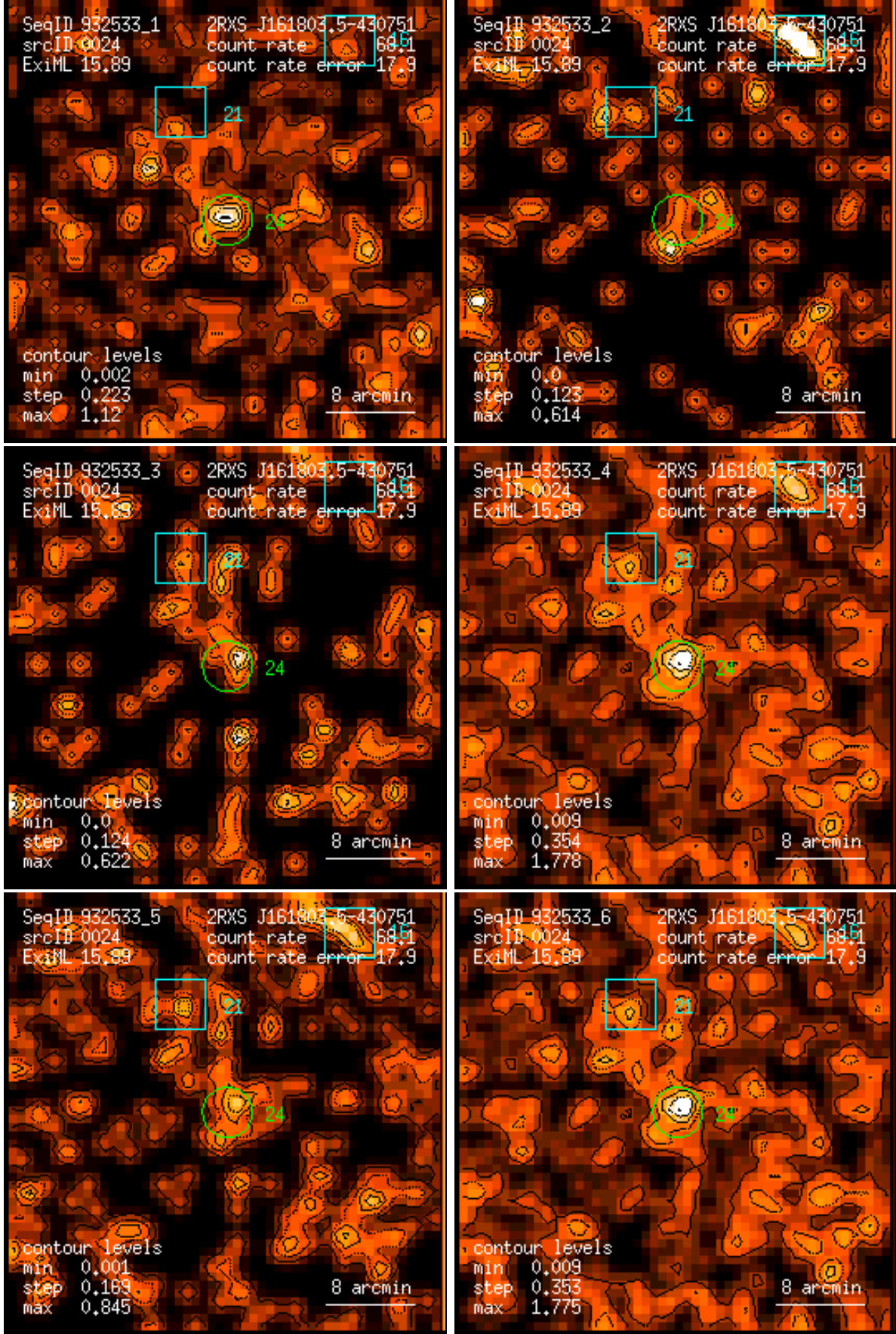
Figure 24: RASS 932533: detection 0024: band rate images, Gaussian filter: (1) PSPC channels 11 – 41, (2) 52 – 90, (3) 91 – 201, (4) 11 – 235, (5) 52 – 201, (6) 11 – 201. Broad band rates in counts/ks. Band rate contour levels in counts/ks/arcmin 2 .
