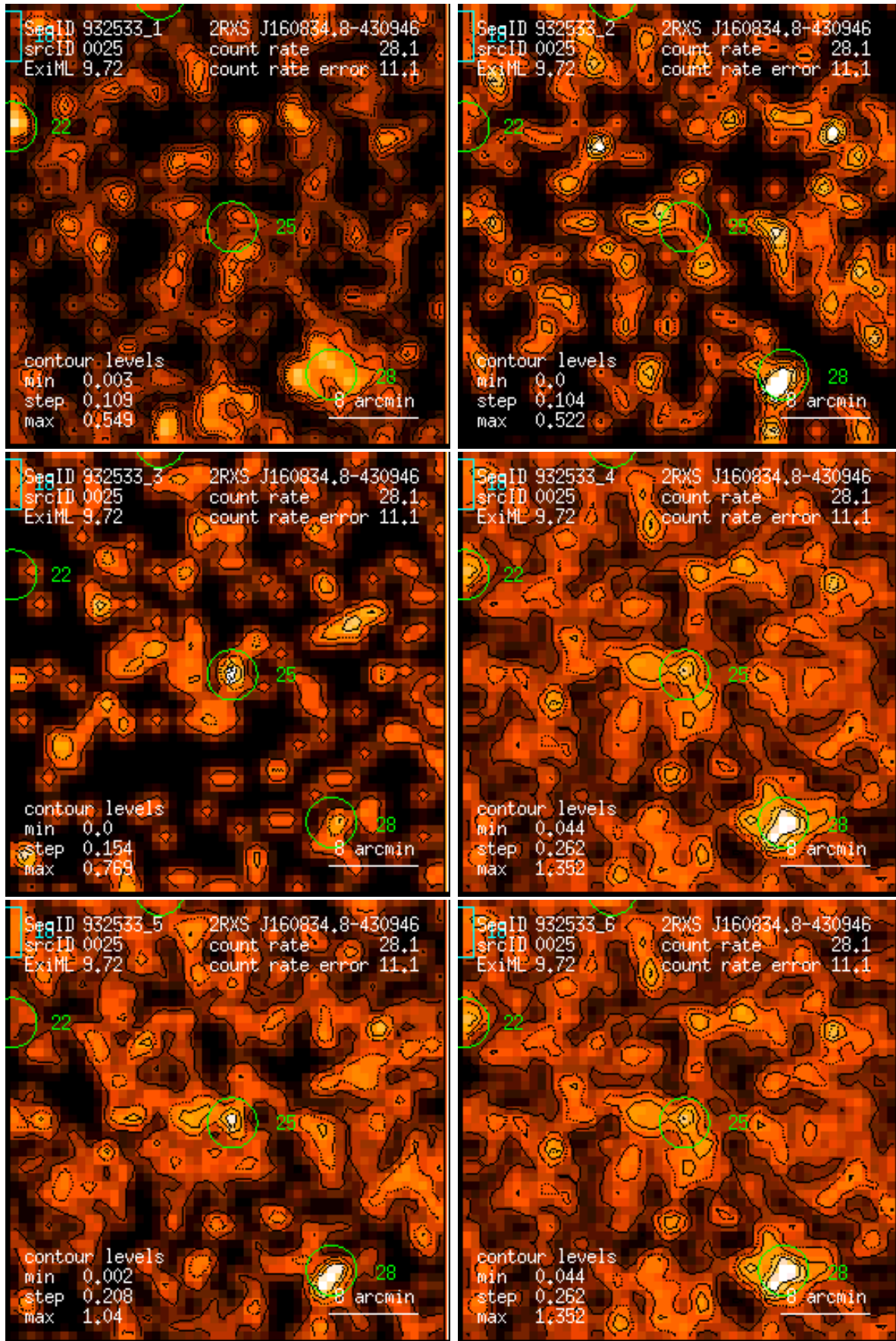
Figure 25: RASS 932533: detection 0025: band rate images, Gaussian filter: (1) PSPC channels 11 – 41, (2) 52 – 90, (3) 91 – 201, (4) 11 – 235, (5) 52 – 201, (6) 11 – 201. Broad band rates in counts/ks. Band rate contour levels in counts/ks/arcmin 2 .
