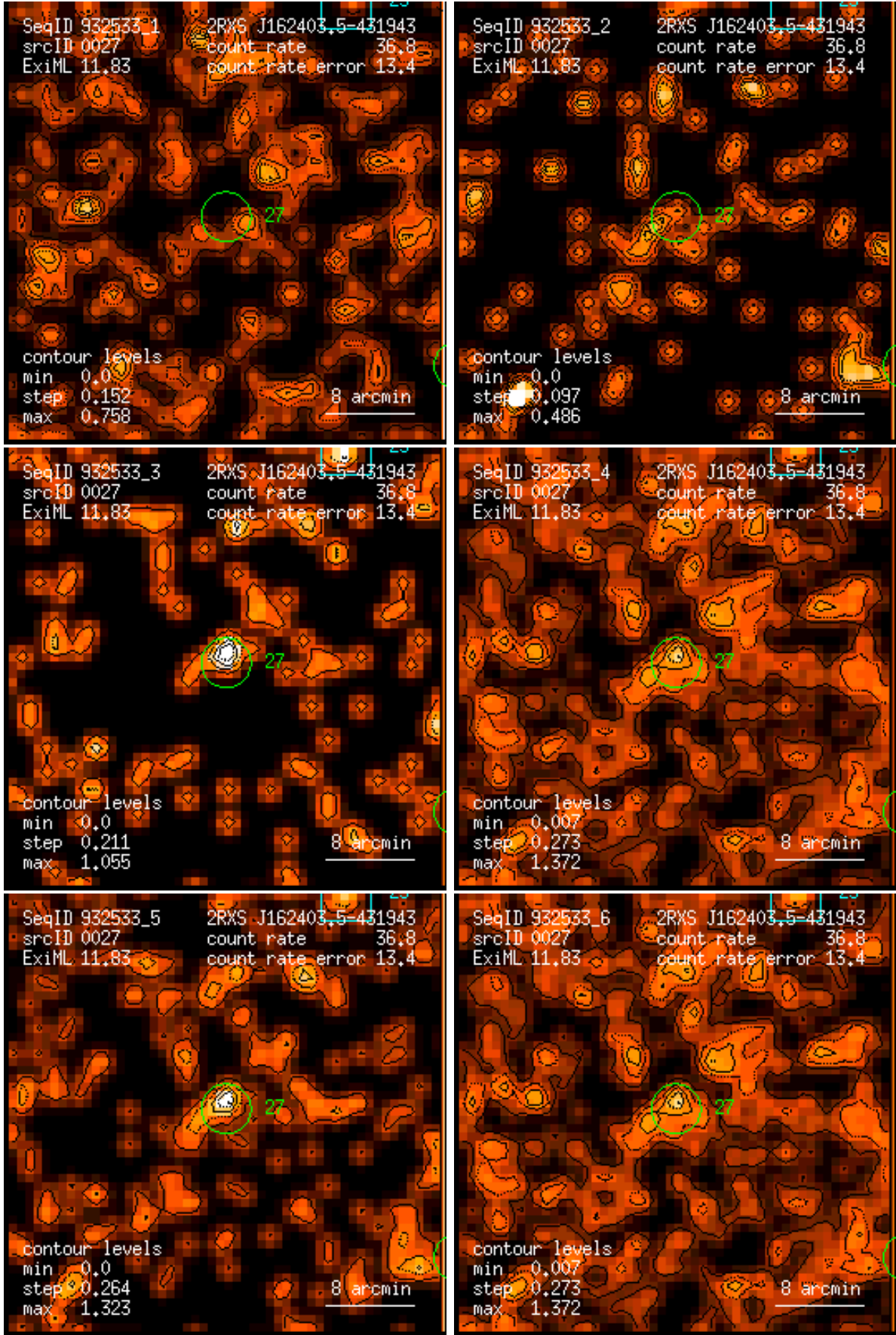
Figure 27: RASS 932533: detection 0027: band rate images, Gaussian filter: (1) PSPC channels 11 – 41, (2) 52 – 90, (3) 91 – 201, (4) 11 – 235, (5) 52 – 201, (6) 11 – 201. Broad band rates in counts/ks. Band rate contour levels in counts/ks/arcmin 2 .
