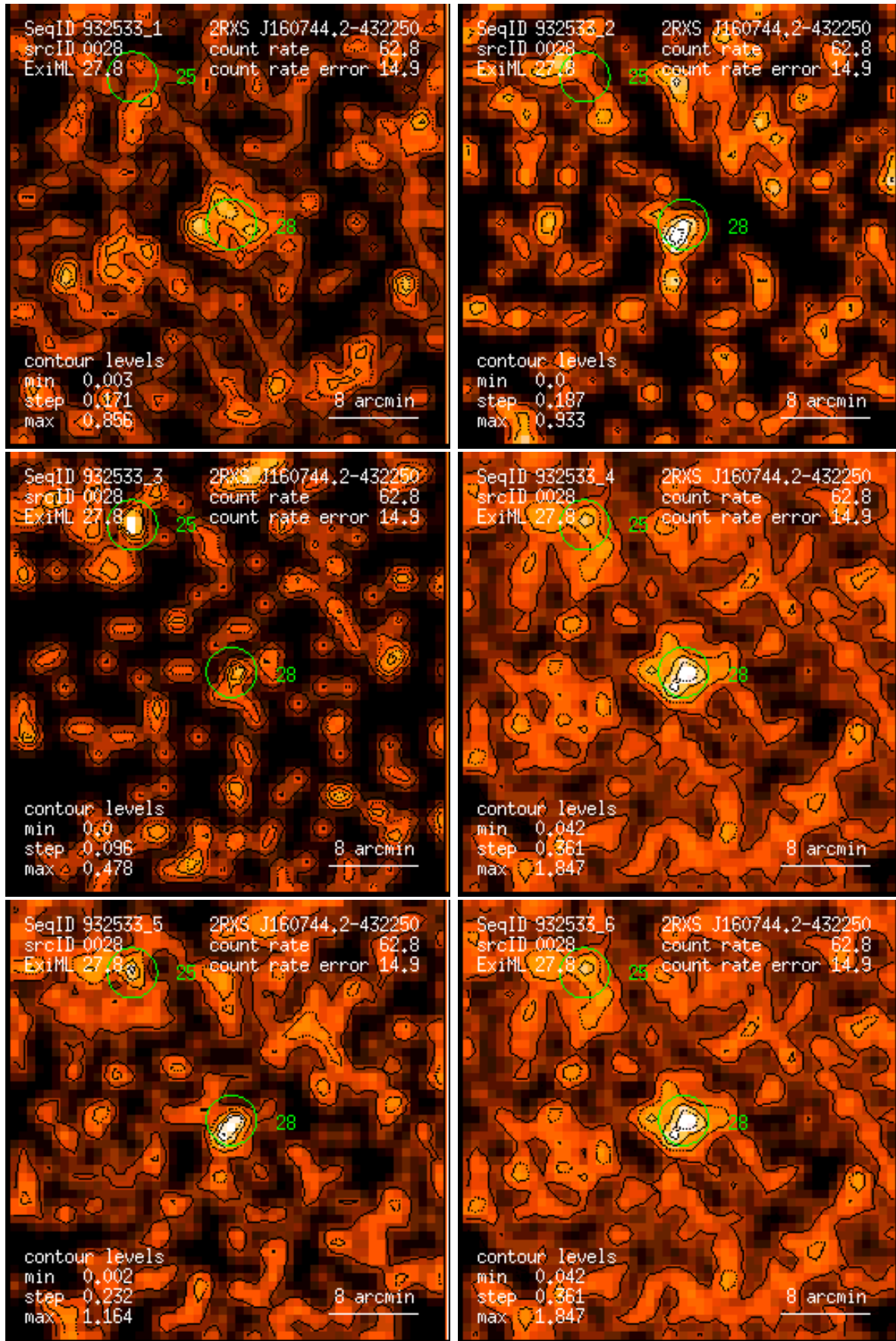
Figure 28: RASS 932533: detection 0028: band rate images, Gaussian filter: (1) PSPC channels 11 – 41, (2) 52 – 90, (3) 91 – 201, (4) 11 – 235, (5) 52 – 201, (6) 11 – 201. Broad band rates in counts/ks. Band rate contour levels in counts/ks/arcmin 2 .
