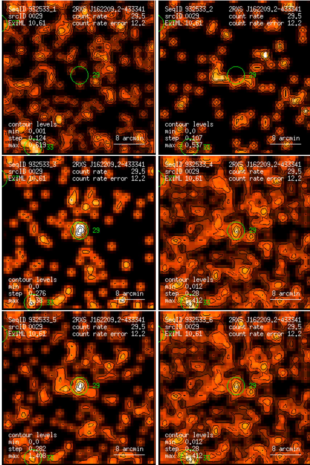
Figure 29: RASS 932533: detection 0029: band rate images, Gaussian filter: (1) PSPC channels 11 – 41, (2) 52 – 90, (3) 91 – 201, (4) 11 – 235, (5) 52 – 201, (6) 11 – 201. Broad band rates in counts/ks. Band rate contour levels in counts/ks/arcmin 2 .
