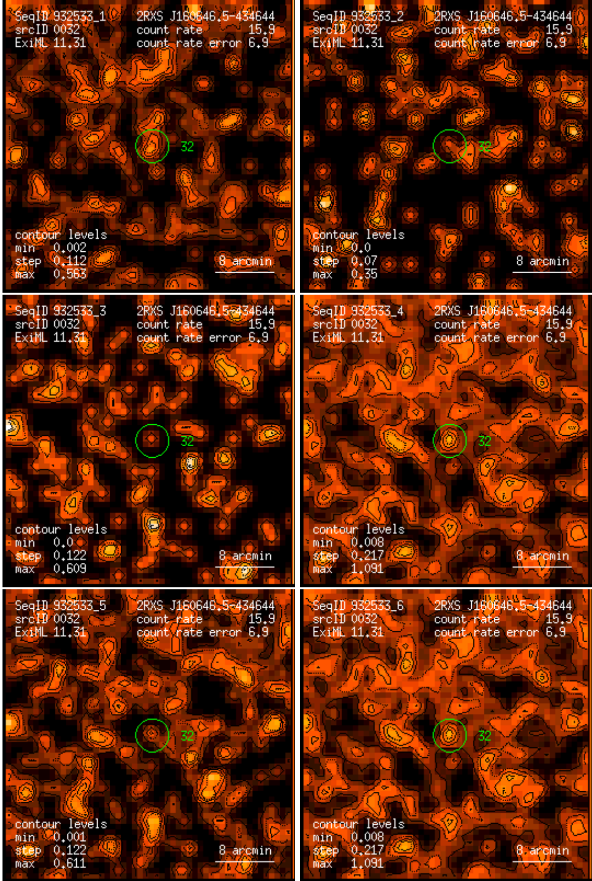
Figure 32: RASS 932533: detection 0032: band rate images, Gaussian filter: (1) PSPC channels 11 – 41, (2) 52 – 90, (3) 91 – 201, (4) 11 – 235, (5) 52 – 201, (6) 11 – 201. Broad band rates in counts/ks. Band rate contour levels in counts/ks/arcmin 2 .
