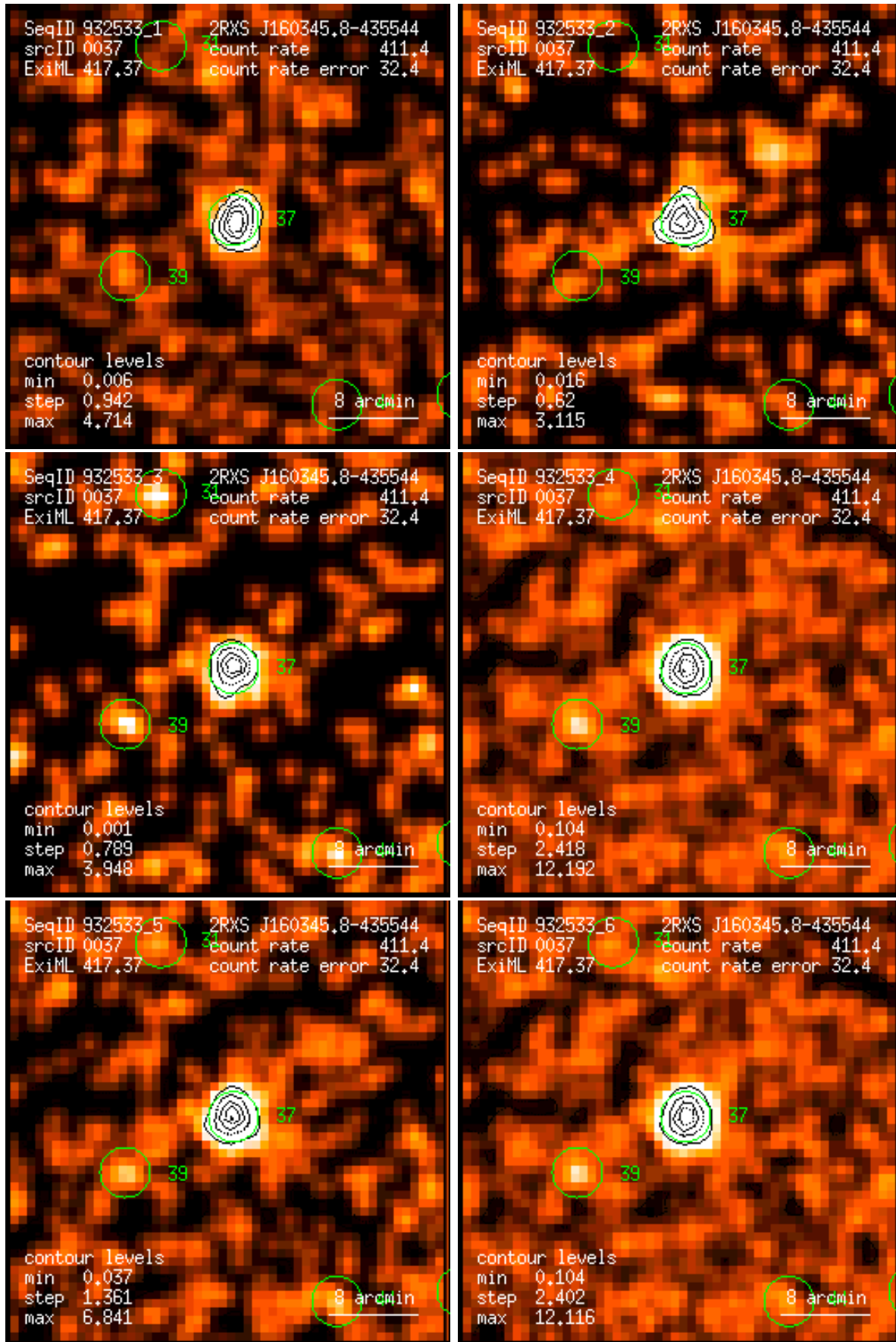
Figure 37: RASS 932533: detection 0037: band rate images, Gaussian filter: (1) PSPC channels 11 – 41, (2) 52 – 90, (3) 91 – 201, (4) 11 – 235, (5) 52 – 201, (6) 11 – 201. Broad band rates in counts/ks. Band rate contour levels in counts/ks/arcmin 2 .
