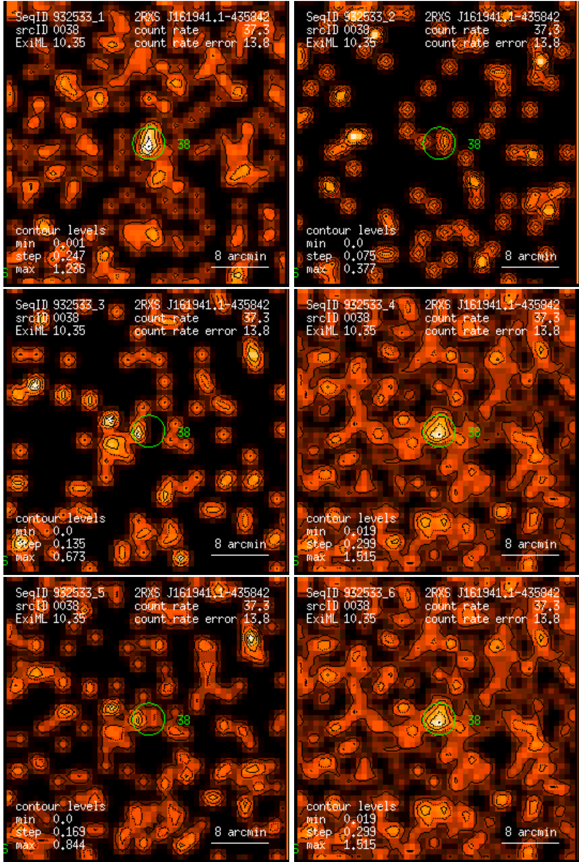
Figure 38: RASS 932533: detection 0038: band rate images, Gaussian filter: (1) PSPC channels 11 – 41, (2) 52 – 90, (3) 91 – 201, (4) 11 – 235, (5) 52 – 201, (6) 11 – 201. Broad band rates in counts/ks. Band rate contour levels in counts/ks/arcmin 2 .
