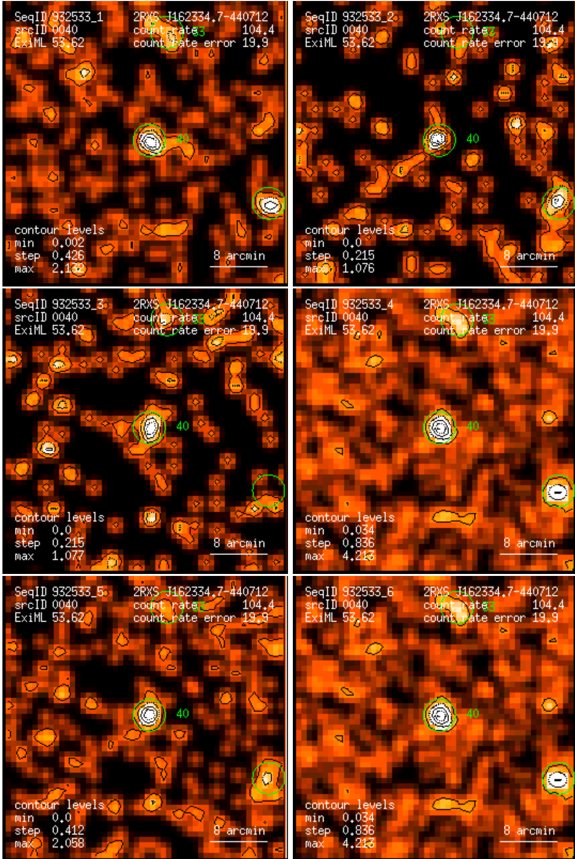
Figure 40: RASS 932533: detection 0040: band rate images, Gaussian filter: (1) PSPC channels 11 – 41, (2) 52 – 90, (3) 91 – 201, (4) 11 – 235, (5) 52 – 201, (6) 11 – 201. Broad band rates in counts/ks. Band rate contour levels in counts/ks/arcmin 2 .
