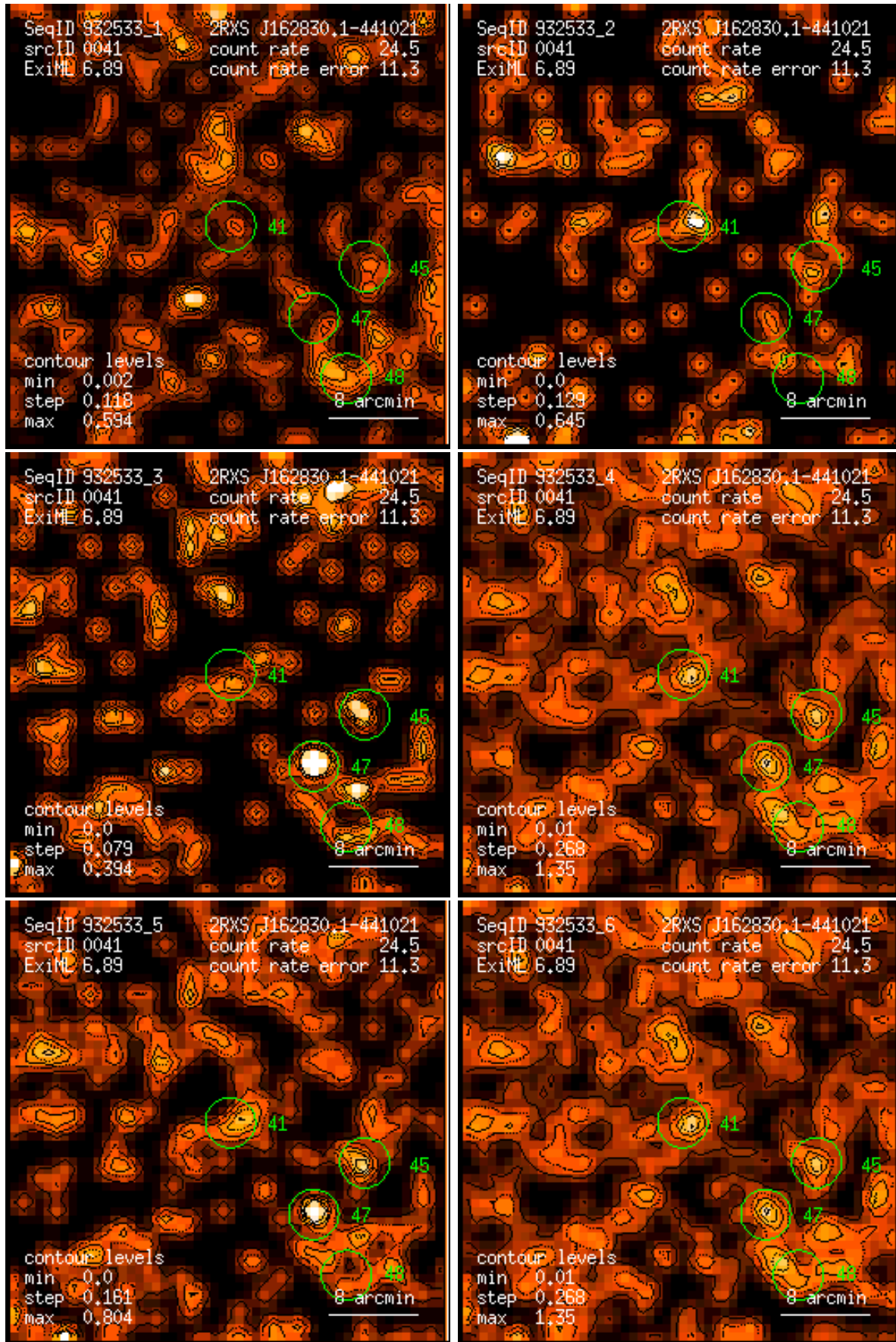
Figure 41: RASS 932533: detection 0041: band rate images, Gaussian filter: (1) PSPC channels 11 – 41, (2) 52 – 90, (3) 91 – 201, (4) 11 – 235, (5) 52 – 201, (6) 11 – 201. Broad band rates in counts/ks. Band rate contour levels in counts/ks/arcmin 2 .
