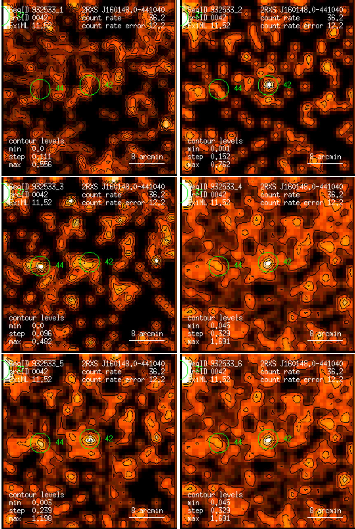
Figure 42: RASS 932533: detection 0042: band rate images, Gaussian filter: (1) PSPC channels 11 – 41, (2) 52 – 90, (3) 91 – 201, (4) 11 – 235, (5) 52 – 201, (6) 11 – 201. Broad band rates in counts/ks. Band rate contour levels in counts/ks/arcmin 2 .
