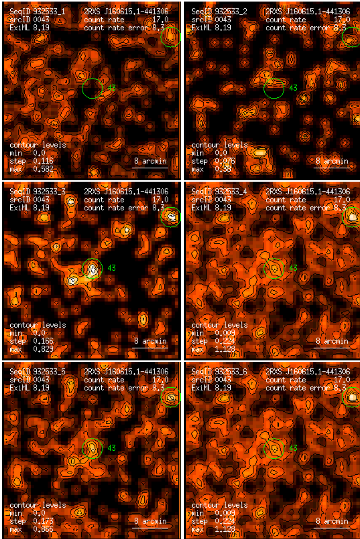
Figure 43: RASS 932533: detection 0043: band rate images, Gaussian filter: (1) PSPC channels 11 – 41, (2) 52 – 90, (3) 91 – 201, (4) 11 – 235, (5) 52 – 201, (6) 11 – 201. Broad band rates in counts/ks. Band rate contour levels in counts/ks/arcmin 2 .
