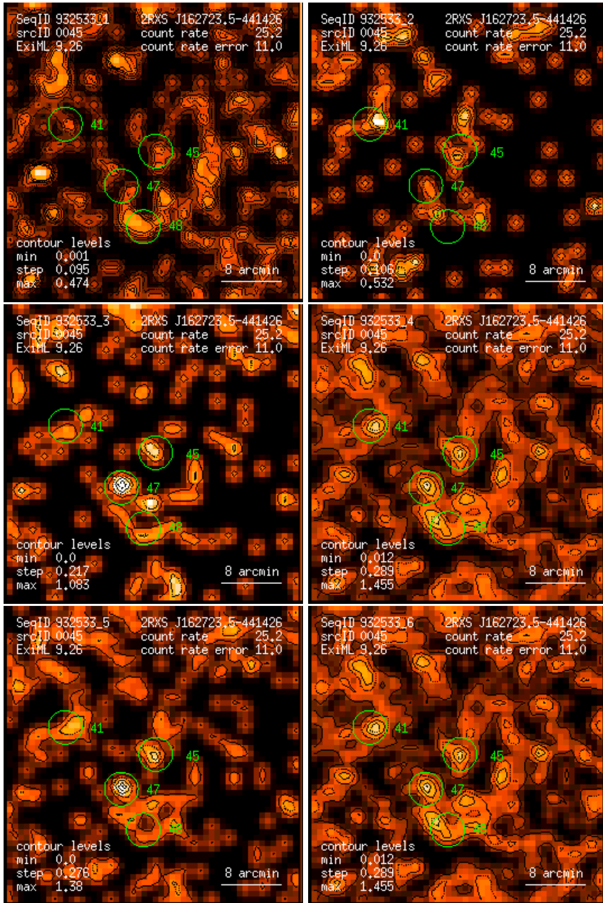
Figure 45: RASS 932533: detection 0045: band rate images, Gaussian filter: (1) PSPC channels 11 – 41, (2) 52 – 90, (3) 91 – 201, (4) 11 – 235, (5) 52 – 201, (6) 11 – 201. Broad band rates in counts/ks. Band rate contour levels in counts/ks/arcmin 2 .
