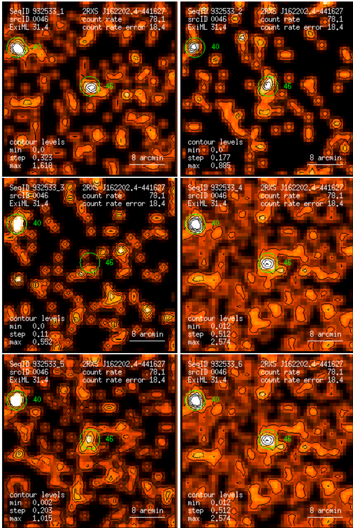
Figure 46: RASS 932533: detection 0046: band rate images, Gaussian filter: (1) PSPC channels 11 – 41, (2) 52 – 90, (3) 91 – 201, (4) 11 – 235, (5) 52 – 201, (6) 11 – 201. Broad band rates in counts/ks. Band rate contour levels in counts/ks/arcmin 2 .
