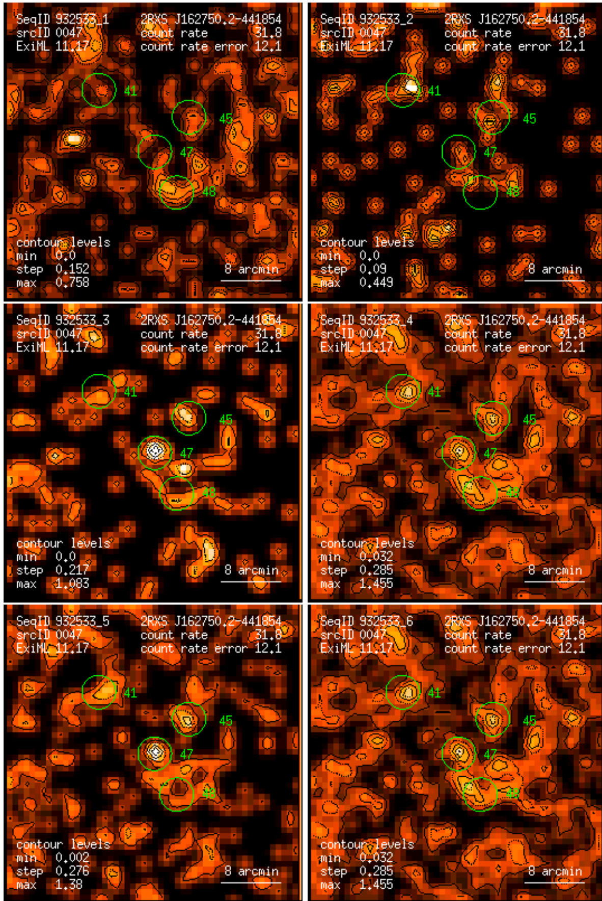
Figure 47: RASS 932533: detection 0047: band rate images, Gaussian filter: (1) PSPC channels 11 – 41, (2) 52 – 90, (3) 91 – 201, (4) 11 – 235, (5) 52 – 201, (6) 11 – 201. Broad band rates in counts/ks. Band rate contour levels in counts/ks/arcmin 2 .
