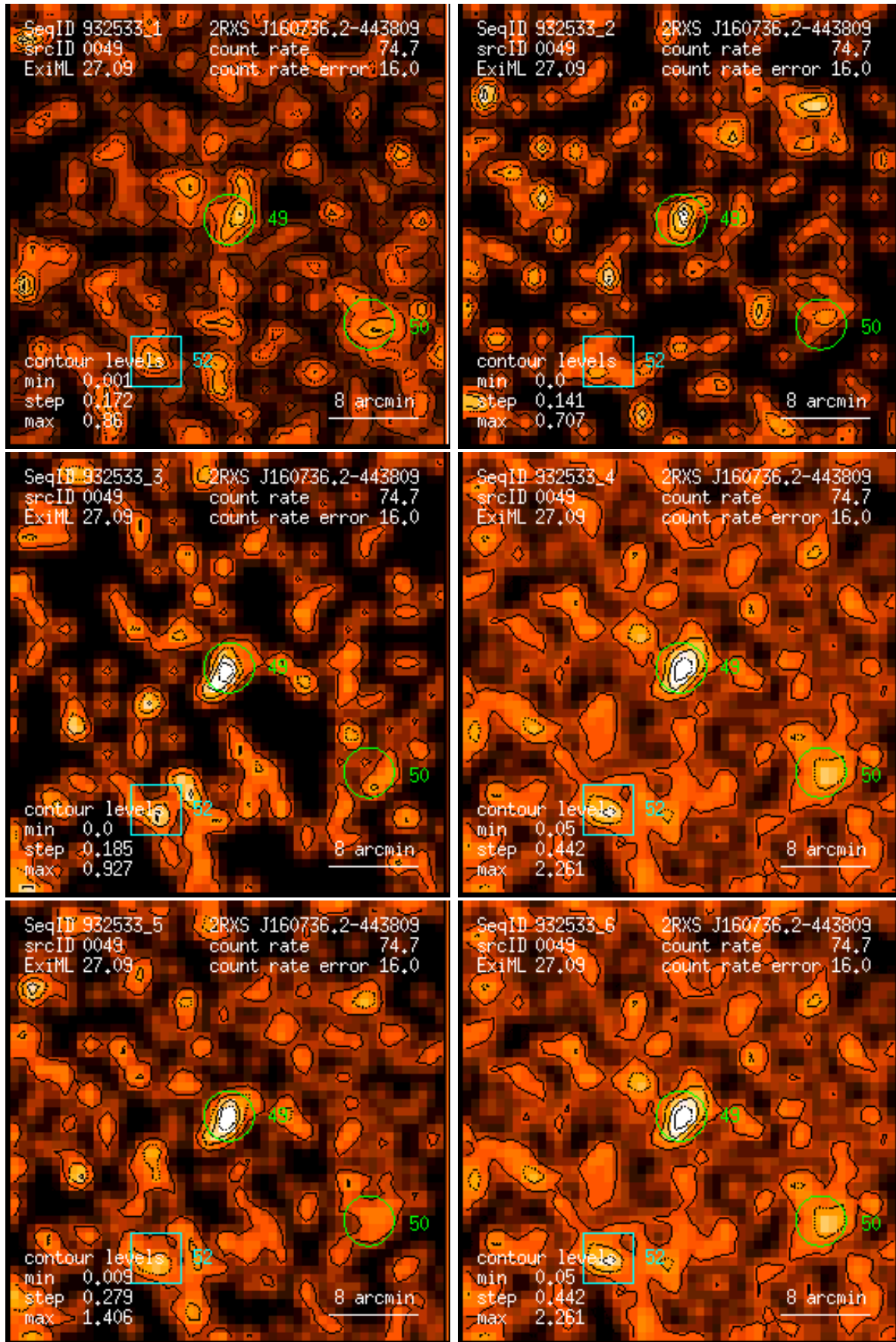
Figure 49: RASS 932533: detection 0049: band rate images, Gaussian filter: (1) PSPC channels 11 – 41, (2) 52 – 90, (3) 91 – 201, (4) 11 – 235, (5) 52 – 201, (6) 11 – 201. Broad band rates in counts/ks. Band rate contour levels in counts/ks/arcmin 2 .
