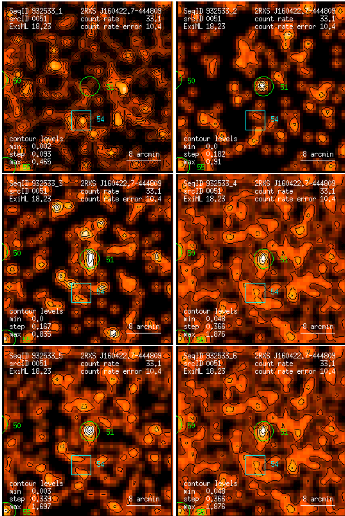
Figure 51: RASS 932533: detection 0051: band rate images, Gaussian filter: (1) PSPC channels 11 – 41, (2) 52 – 90, (3) 91 – 201, (4) 11 – 235, (5) 52 – 201, (6) 11 – 201. Broad band rates in counts/ks. Band rate contour levels in counts/ks/arcmin 2 .
