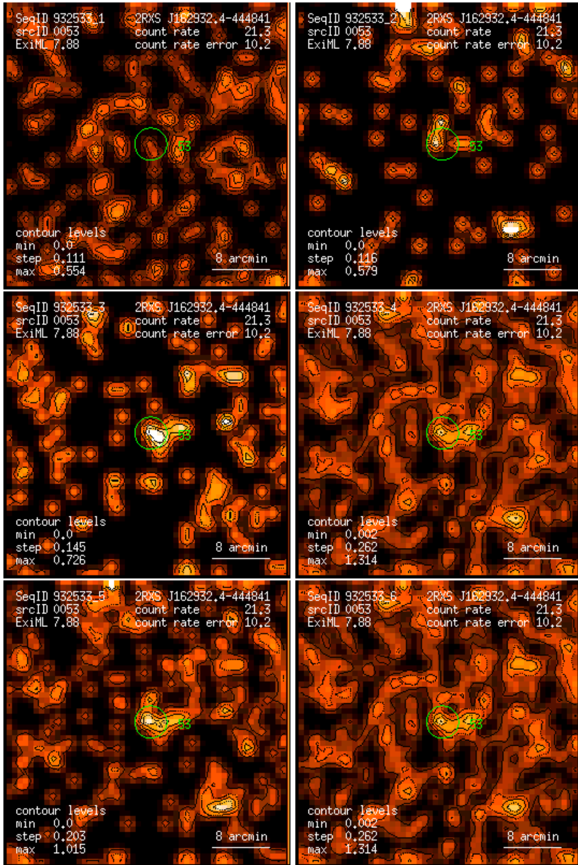
Figure 53: RASS 932533: detection 0053: band rate images, Gaussian filter: (1) PSPC channels 11 – 41, (2) 52 – 90, (3) 91 – 201, (4) 11 – 235, (5) 52 – 201, (6) 11 – 201. Broad band rates in counts/ks. Band rate contour levels in counts/ks/arcmin 2 .
