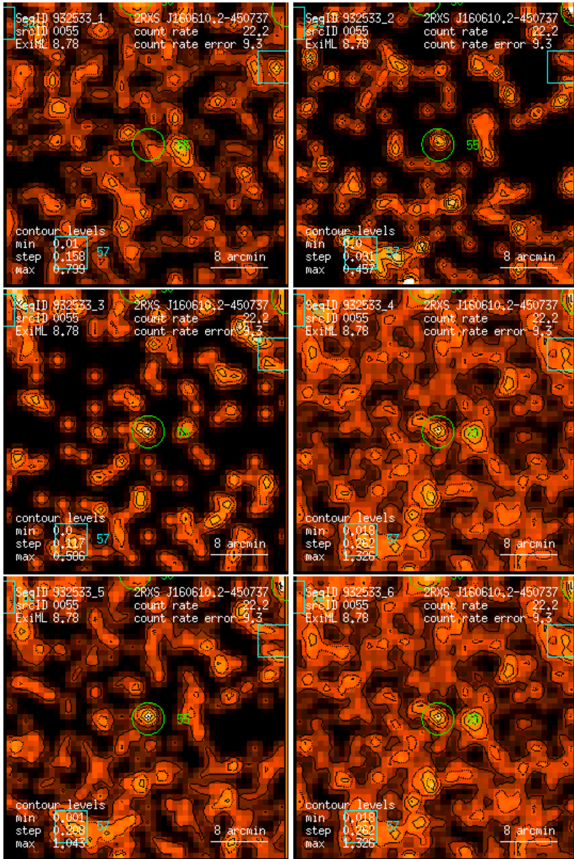
Figure 55: RASS 932533: detection 0055: band rate images, Gaussian filter: (1) PSPC channels 11 – 41, (2) 52 – 90, (3) 91 – 201, (4) 11 – 235, (5) 52 – 201, (6) 11 – 201. Broad band rates in counts/ks. Band rate contour levels in counts/ks/arcmin 2 .
