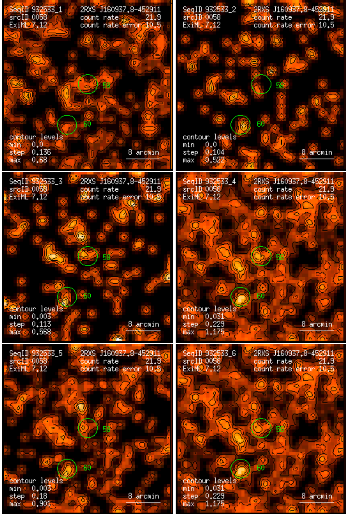
Figure 58: RASS 932533: detection 0058: band rate images, Gaussian filter: (1) PSPC channels 11 – 41, (2) 52 – 90, (3) 91 – 201, (4) 11 – 235, (5) 52 – 201, (6) 11 – 201. Broad band rates in counts/ks. Band rate contour levels in counts/ks/arcmin 2 .
