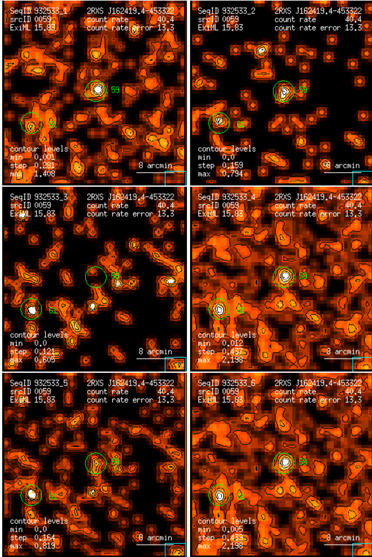
Figure 59: RASS 932533: detection 0059: band rate images, Gaussian filter: (1) PSPC channels 11 – 41, (2) 52 – 90, (3) 91 – 201, (4) 11 – 235, (5) 52 – 201, (6) 11 – 201. Broad band rates in counts/ks. Band rate contour levels in counts/ks/arcmin 2 .
