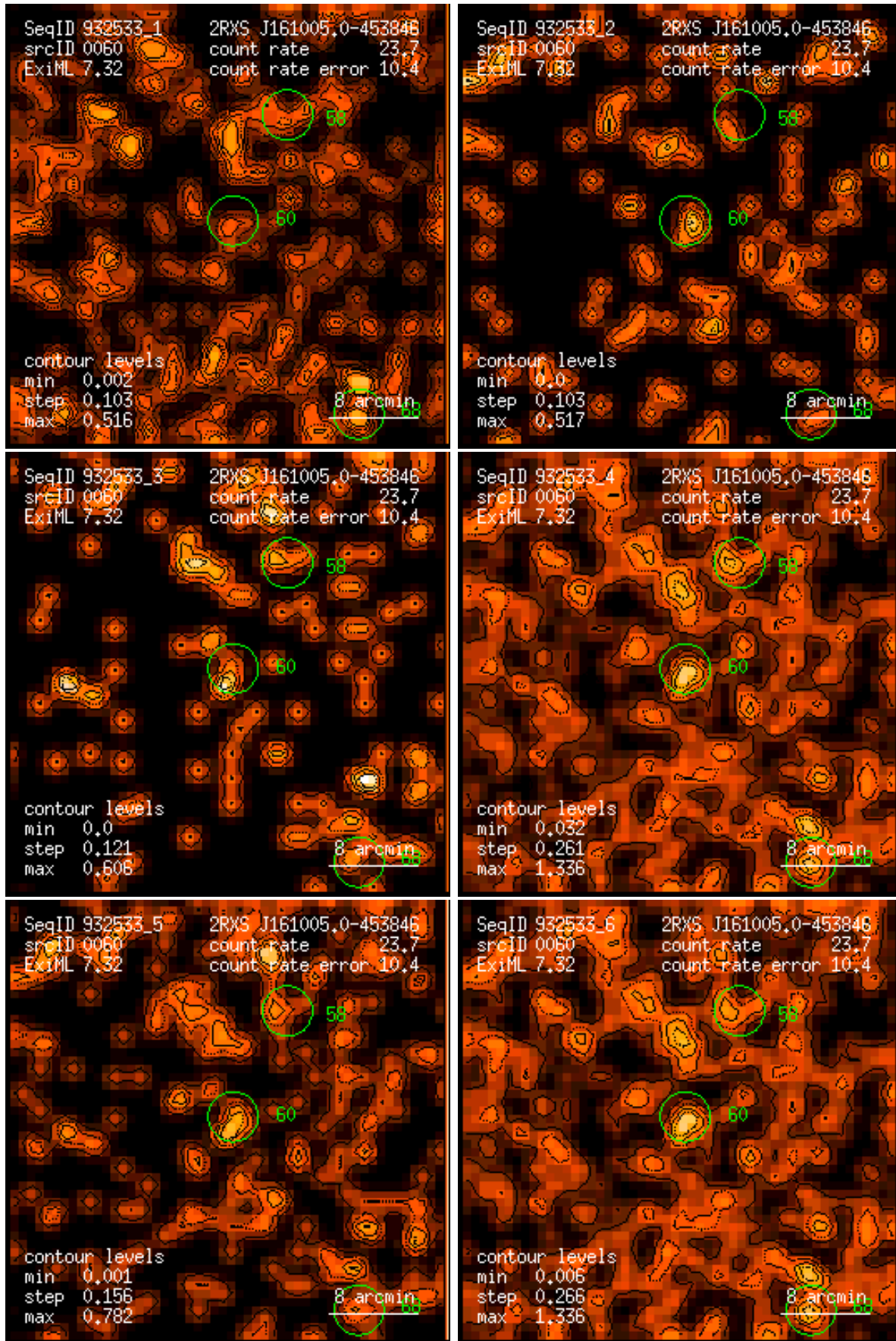
Figure 60: RASS 932533: detection 0060: band rate images, Gaussian filter: (1) PSPC channels 11 – 41, (2) 52 – 90, (3) 91 – 201, (4) 11 – 235, (5) 52 – 201, (6) 11 – 201. Broad band rates in counts/ks. Band rate contour levels in counts/ks/arcmin 2 .
