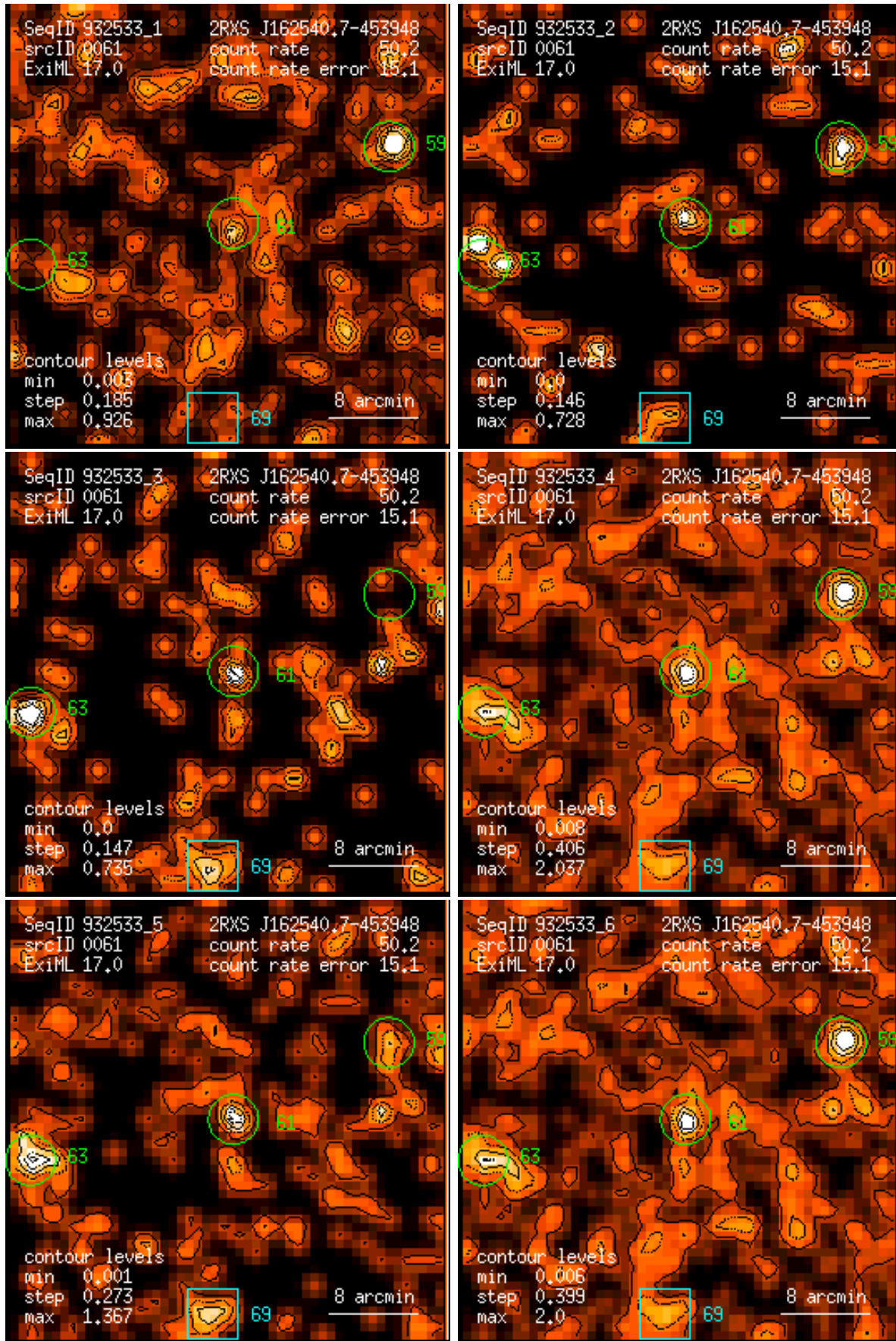
Figure 61: RASS 932533: detection 0061: band rate images, Gaussian filter: (1) PSPC channels 11 – 41, (2) 52 – 90, (3) 91 – 201, (4) 11 – 235, (5) 52 – 201, (6) 11 – 201. Broad band rates in counts/ks. Band rate contour levels in counts/ks/arcmin 2 .
