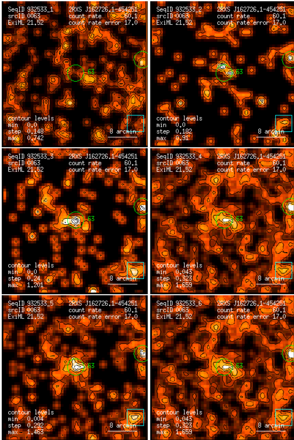
Figure 63: RASS 932533: detection 0063: band rate images, Gaussian filter: (1) PSPC channels 11 – 41, (2) 52 – 90, (3) 91 – 201, (4) 11 – 235, (5) 52 – 201, (6) 11 – 201. Broad band rates in counts/ks. Band rate contour levels in counts/ks/arcmin 2 .
