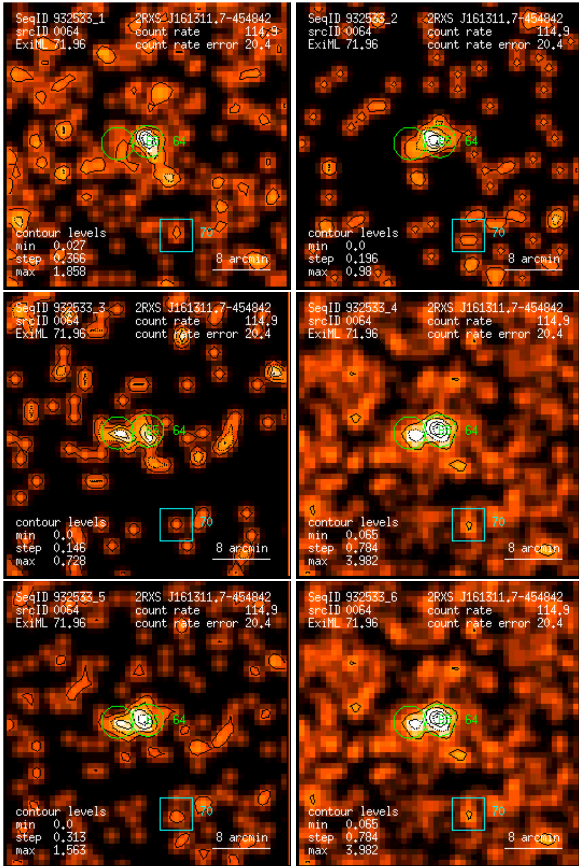
Figure 64: RASS 932533: detection 0064: band rate images, Gaussian filter: (1) PSPC channels 11 – 41, (2) 52 – 90, (3) 91 – 201, (4) 11 – 235, (5) 52 – 201, (6) 11 – 201. Broad band rates in counts/ks. Band rate contour levels in counts/ks/arcmin 2 .
