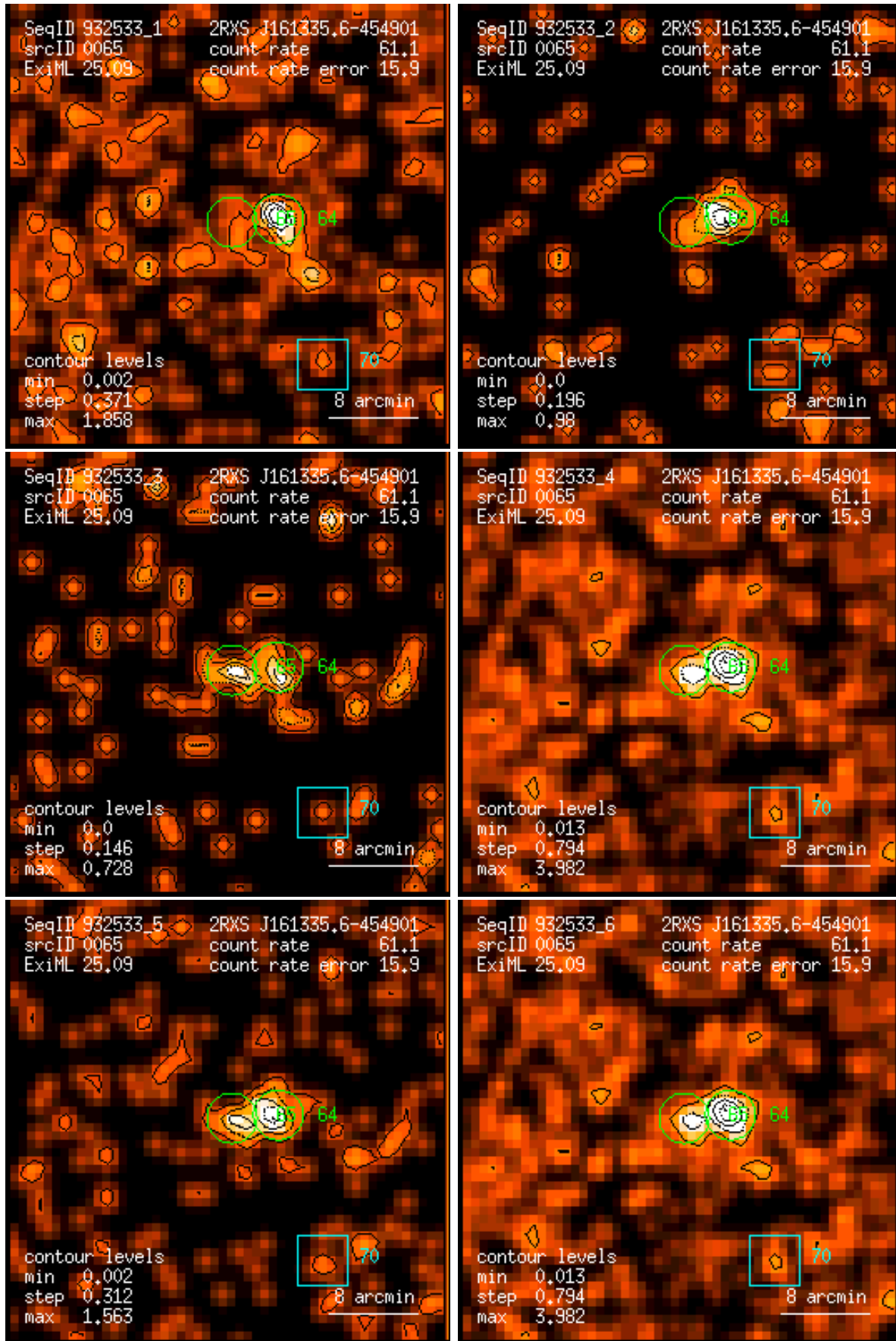
Figure 65: RASS 932533: detection 0065: band rate images, Gaussian filter: (1) PSPC channels 11 – 41, (2) 52 – 90, (3) 91 – 201, (4) 11 – 235, (5) 52 – 201, (6) 11 – 201. Broad band rates in counts/ks. Band rate contour levels in counts/ks/arcmin 2 .
