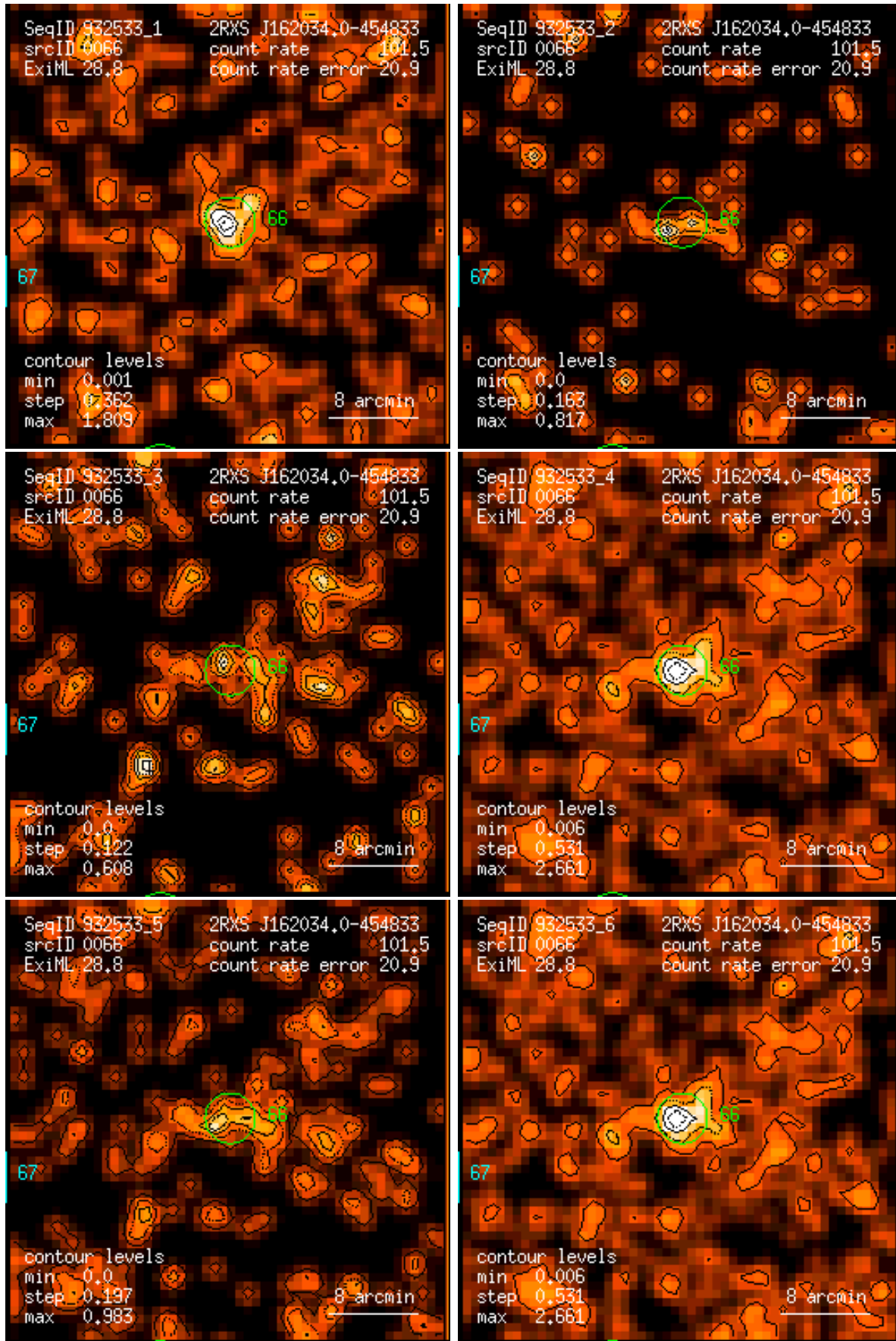
Figure 66: RASS 932533: detection 0066: band rate images, Gaussian filter: (1) PSPC channels 11 – 41, (2) 52 – 90, (3) 91 – 201, (4) 11 – 235, (5) 52 – 201, (6) 11 – 201. Broad band rates in counts/ks. Band rate contour levels in counts/ks/arcmin 2 .
