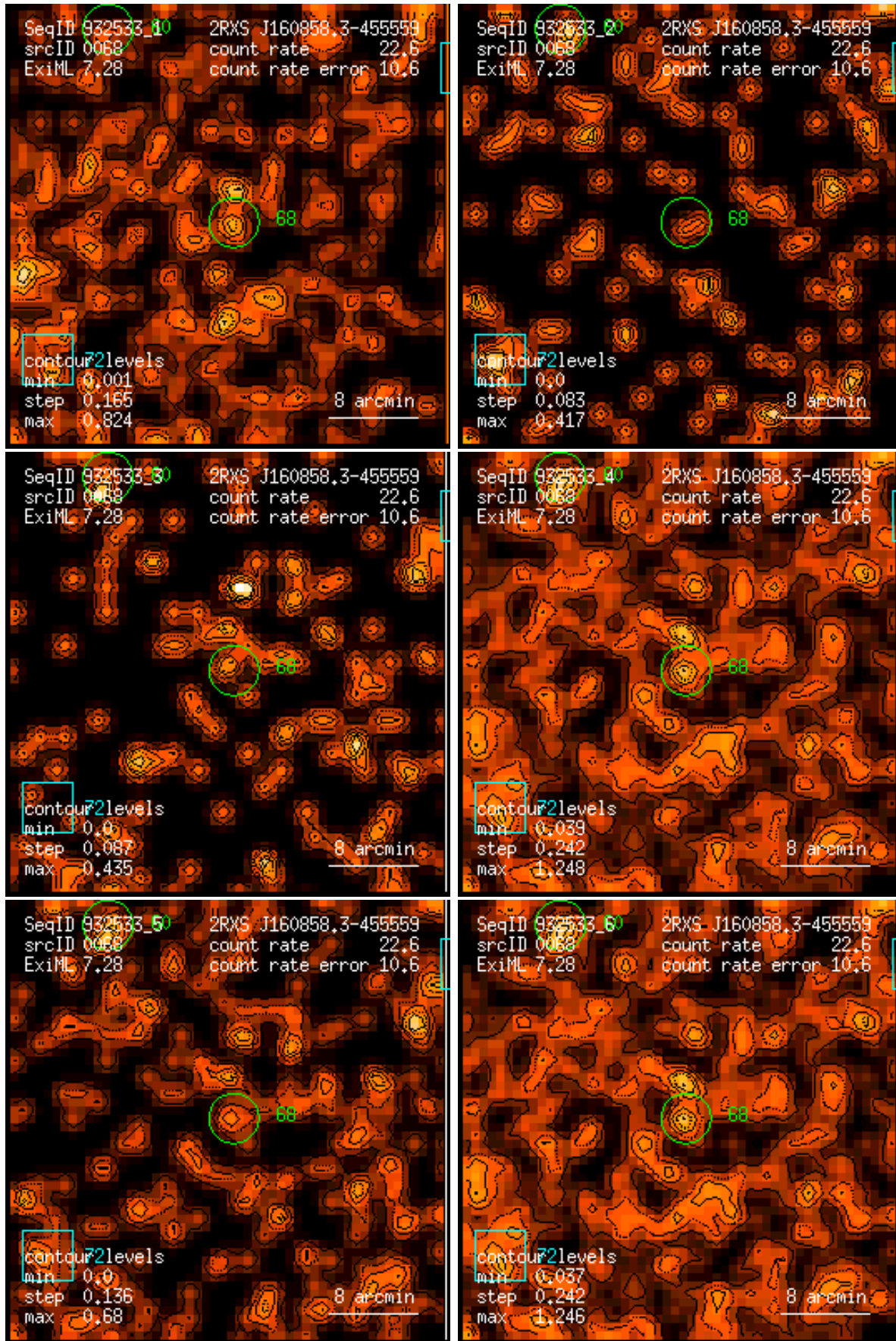
Figure 68: RASS 932533: detection 0068: band rate images, Gaussian filter: (1) PSPC channels 11 – 41, (2) 52 – 90, (3) 91 – 201, (4) 11 – 235, (5) 52 – 201, (6) 11 – 201. Broad band rates in counts/ks. Band rate contour levels in counts/ks/arcmin 2 .
