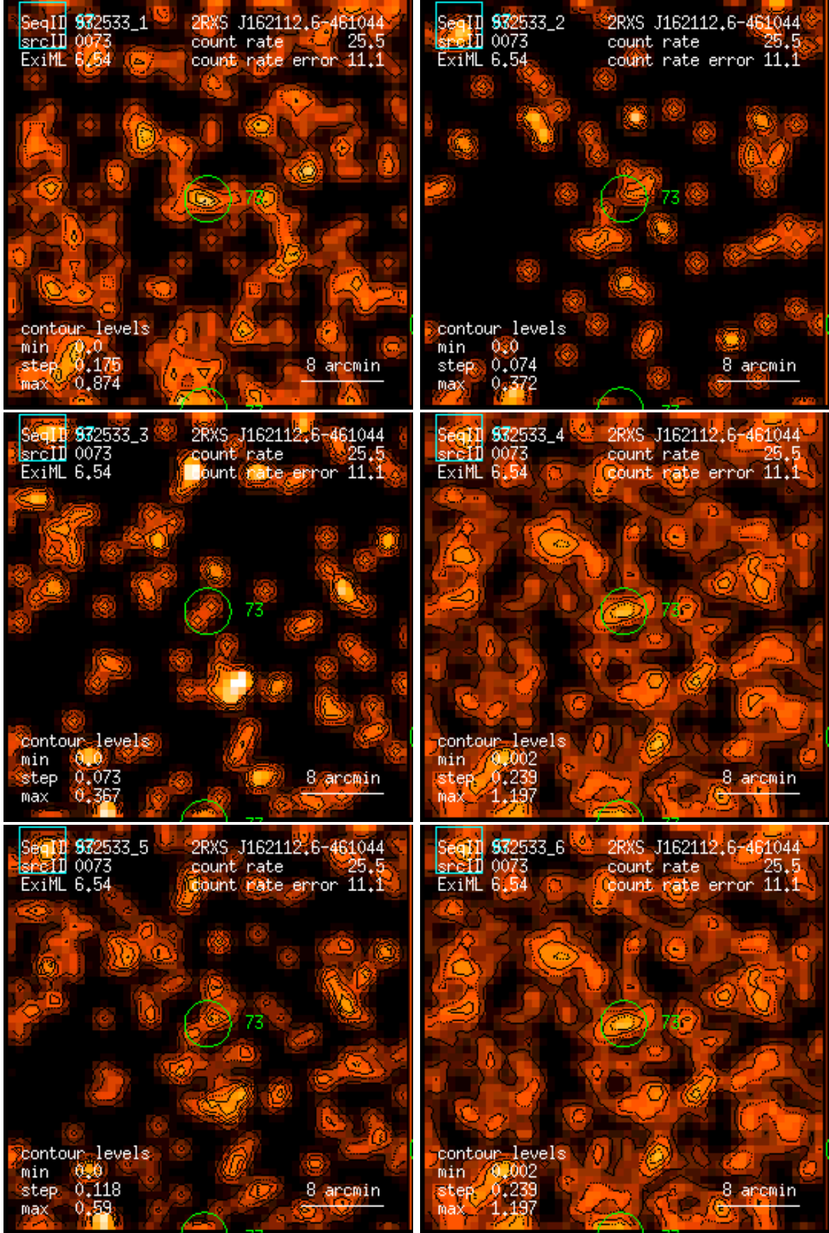
Figure 73: RASS 932533: detection 0073: band rate images, Gaussian filter: (1) PSPC channels 11 – 41, (2) 52 – 90, (3) 91 – 201, (4) 11 – 235, (5) 52 – 201, (6) 11 – 201. Broad band rates in counts/ks. Band rate contour levels in counts/ks/arcmin 2 .
