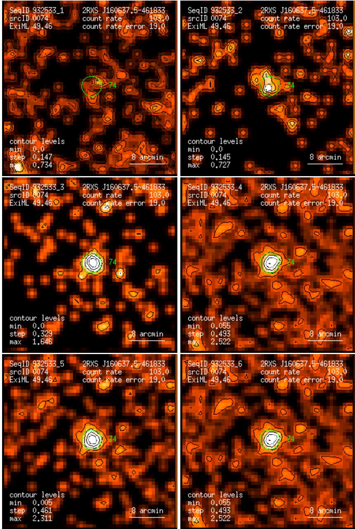
Figure 74: RASS 932533: detection 0074: band rate images, Gaussian filter: (1) PSPC channels 11 – 41, (2) 52 – 90, (3) 91 – 201, (4) 11 – 235, (5) 52 – 201, (6) 11 – 201. Broad band rates in counts/ks. Band rate contour levels in counts/ks/arcmin 2 .
