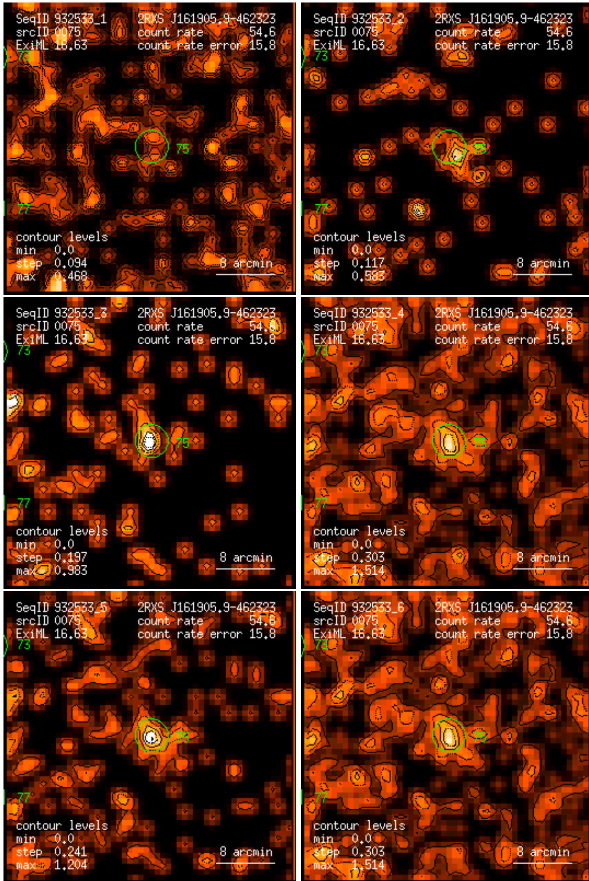
Figure 75: RASS 932533: detection 0075: band rate images, Gaussian filter: (1) PSPC channels 11 – 41, (2) 52 – 90, (3) 91 – 201, (4) 11 – 235, (5) 52 – 201, (6) 11 – 201. Broad band rates in counts/ks. Band rate contour levels in counts/ks/arcmin 2 .
