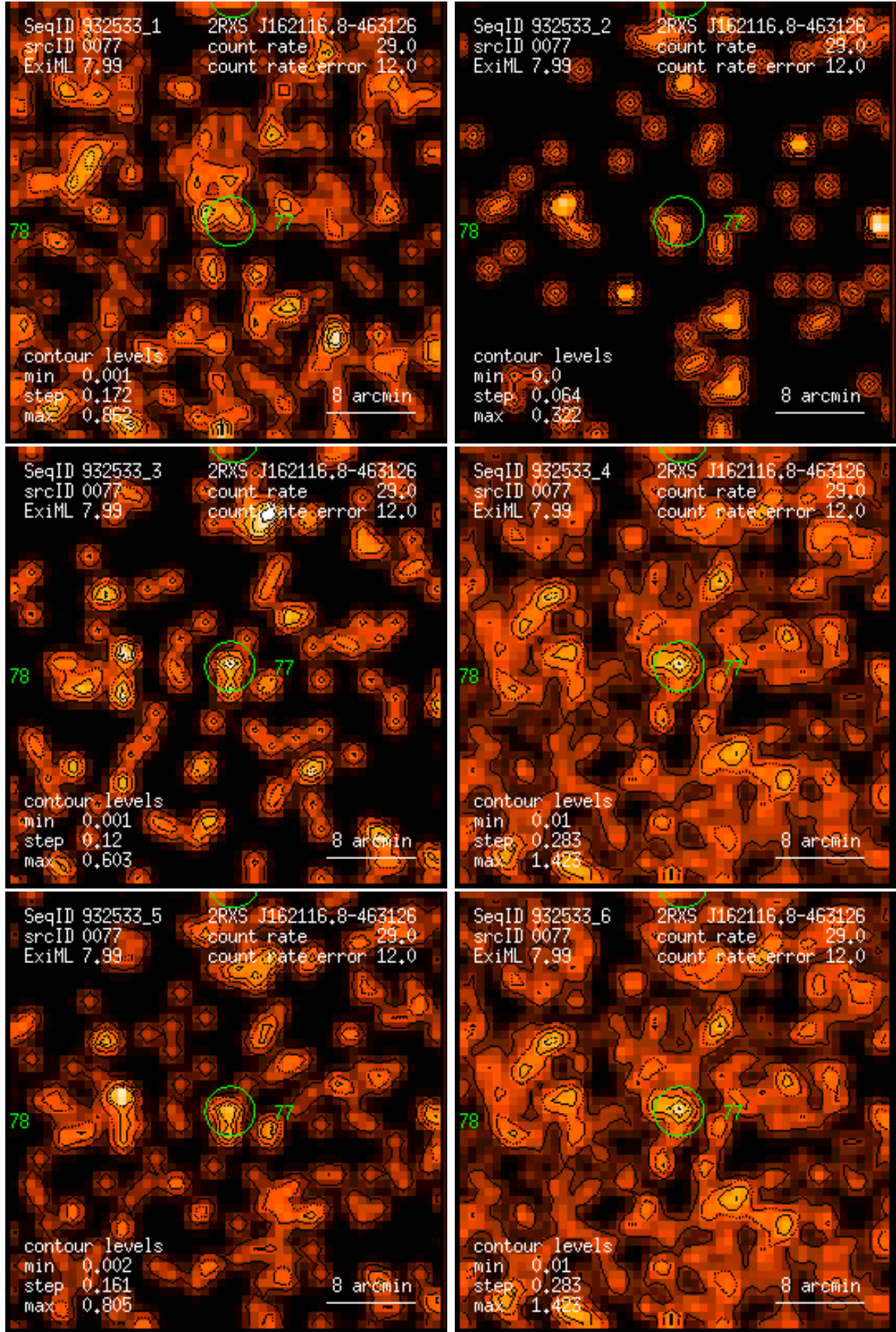
Figure 77: RASS 932533: detection 0077: band rate images, Gaussian filter: (1) PSPC channels 11 – 41, (2) 52 – 90, (3) 91 – 201, (4) 11 – 235, (5) 52 – 201, (6) 11 – 201. Broad band rates in counts/ks. Band rate contour levels in counts/ks/arcmin 2 .
