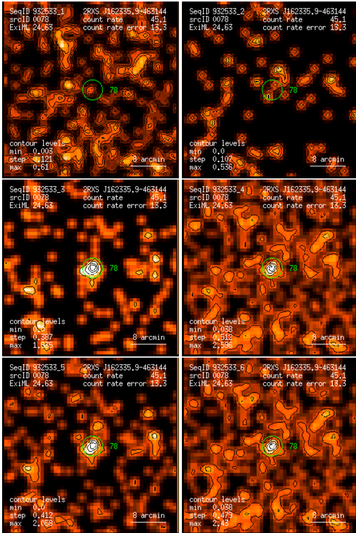
Figure 78: RASS 932533: detection 0078: band rate images, Gaussian filter: (1) PSPC channels 11 – 41, (2) 52 – 90, (3) 91 – 201, (4) 11 – 235, (5) 52 – 201, (6) 11 – 201. Broad band rates in counts/ks. Band rate contour levels in counts/ks/arcmin 2 .
