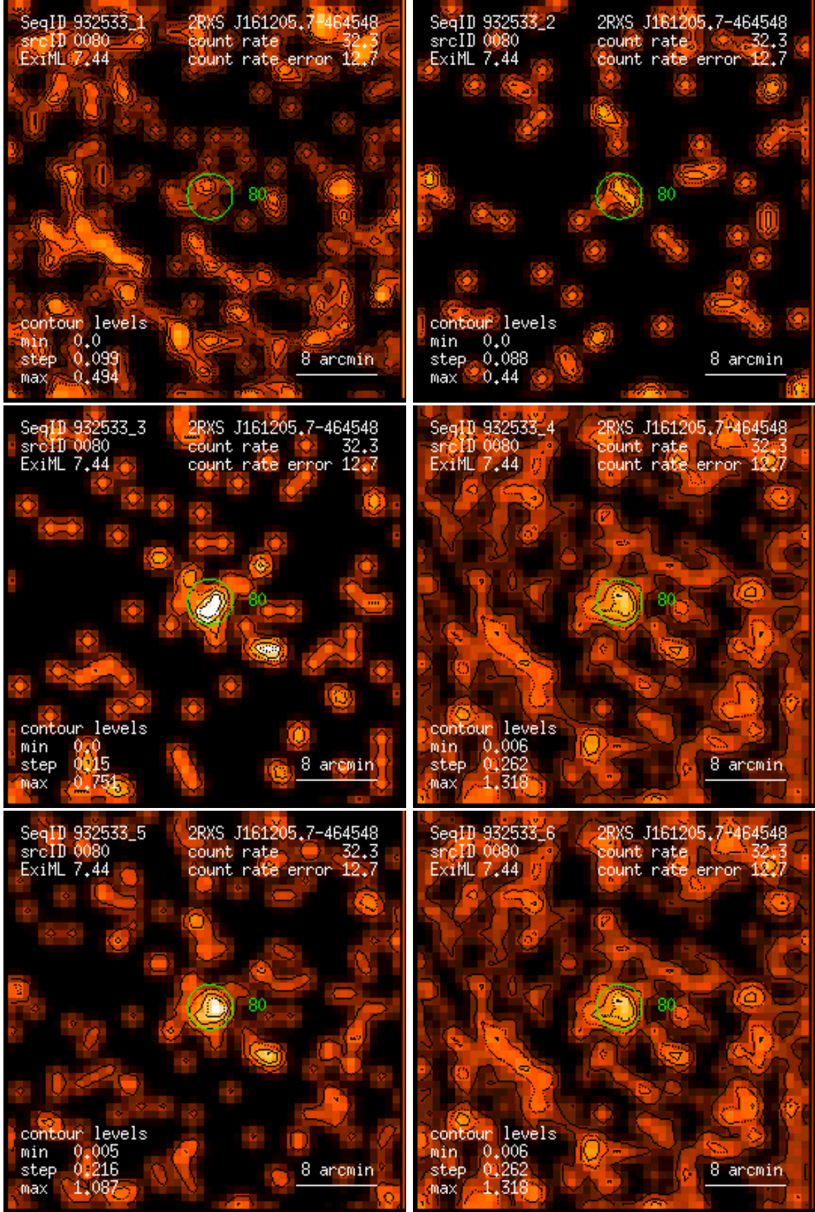
Figure 80: RASS 932533: detection 0080: band rate images, Gaussian filter: (1) PSPC channels 11 – 41, (2) 52 – 90, (3) 91 – 201, (4) 11 – 235, (5) 52 – 201, (6) 11 – 201. Broad band rates in counts/ks. Band rate contour levels in counts/ks/arcmin 2 .
