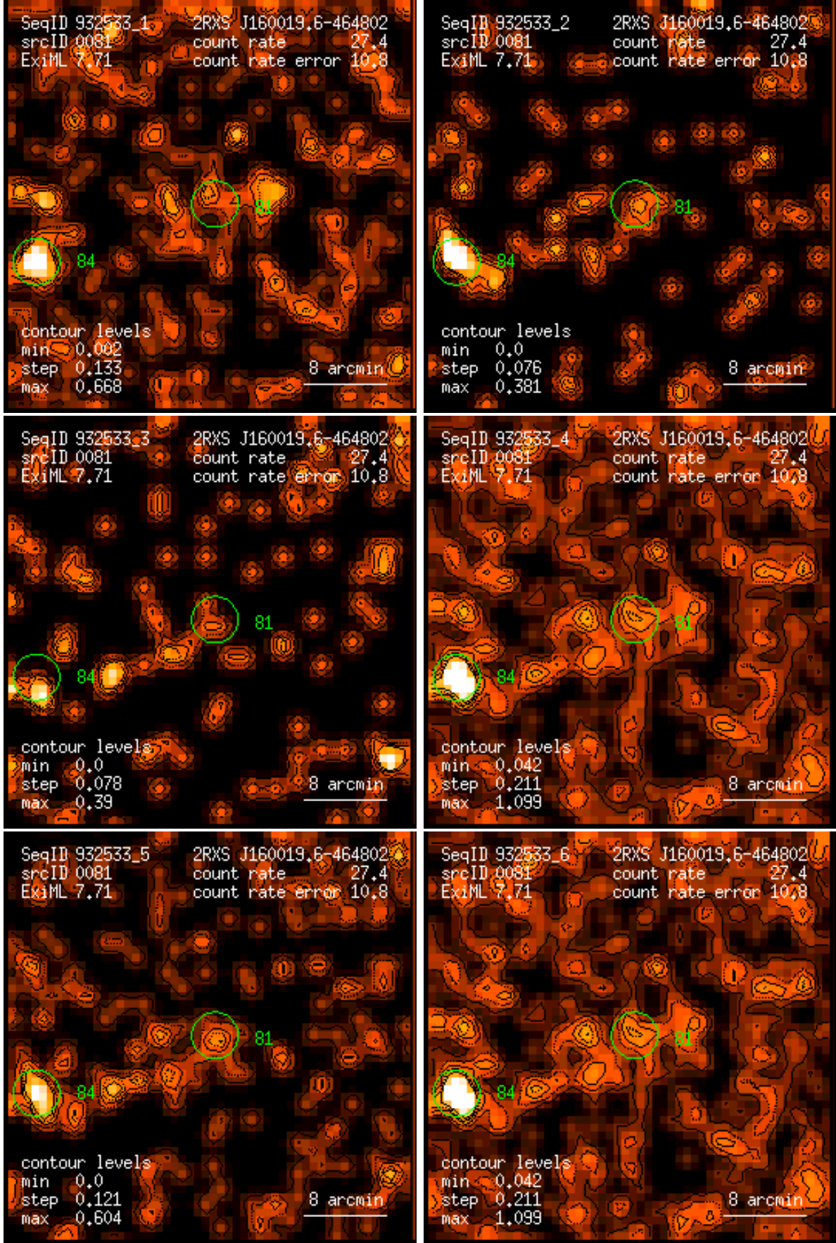
Figure 81: RASS 932533: detection 0081: band rate images, Gaussian filter: (1) PSPC channels 11 – 41, (2) 52 – 90, (3) 91 – 201, (4) 11 – 235, (5) 52 – 201, (6) 11 – 201. Broad band rates in counts/ks. Band rate contour levels in counts/ks/arcmin 2 .
