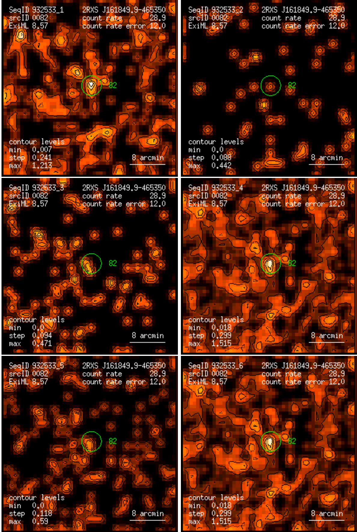
Figure 82: RASS 932533: detection 0082: band rate images, Gaussian filter: (1) PSPC channels 11 – 41, (2) 52 – 90, (3) 91 – 201, (4) 11 – 235, (5) 52 – 201, (6) 11 – 201. Broad band rates in counts/ks. Band rate contour levels in counts/ks/arcmin 2 .
