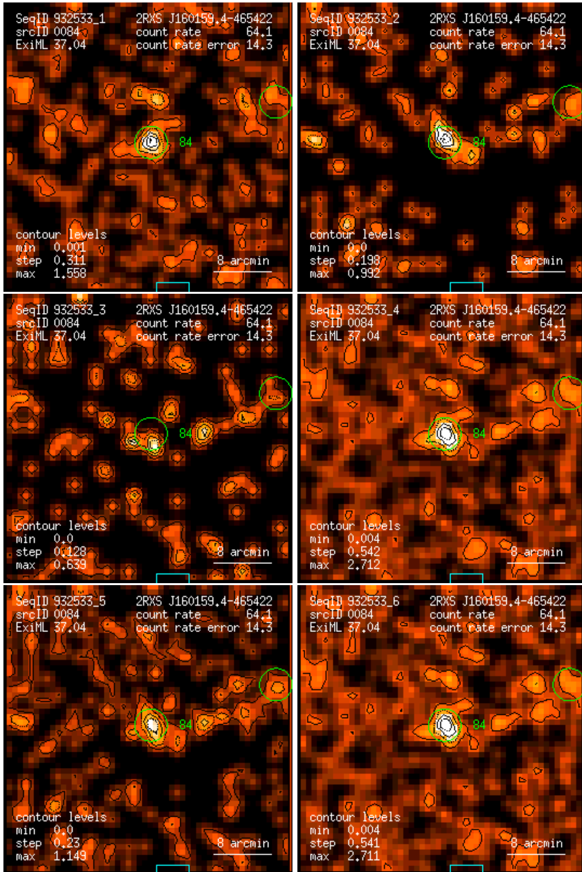
Figure 84: RASS 932533: detection 0084: band rate images, Gaussian filter: (1) PSPC channels 11 – 41, (2) 52 – 90, (3) 91 – 201, (4) 11 – 235, (5) 52 – 201, (6) 11 – 201. Broad band rates in counts/ks. Band rate contour levels in counts/ks/arcmin 2 .
