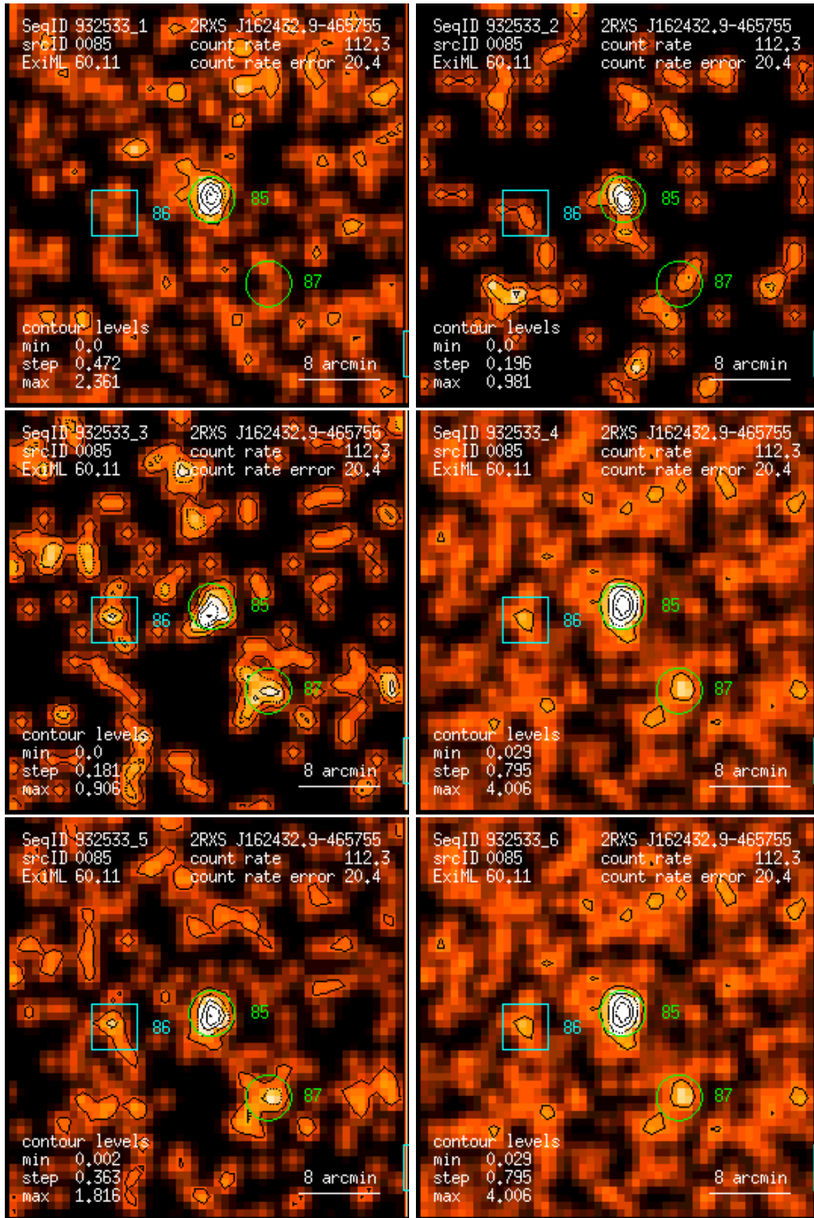
Figure 85: RASS 932533: detection 0085: band rate images, Gaussian filter: (1) PSPC channels 11 – 41, (2) 52 – 90, (3) 91 – 201, (4) 11 – 235, (5) 52 – 201, (6) 11 – 201. Broad band rates in counts/ks. Band rate contour levels in counts/ks/arcmin 2 .
