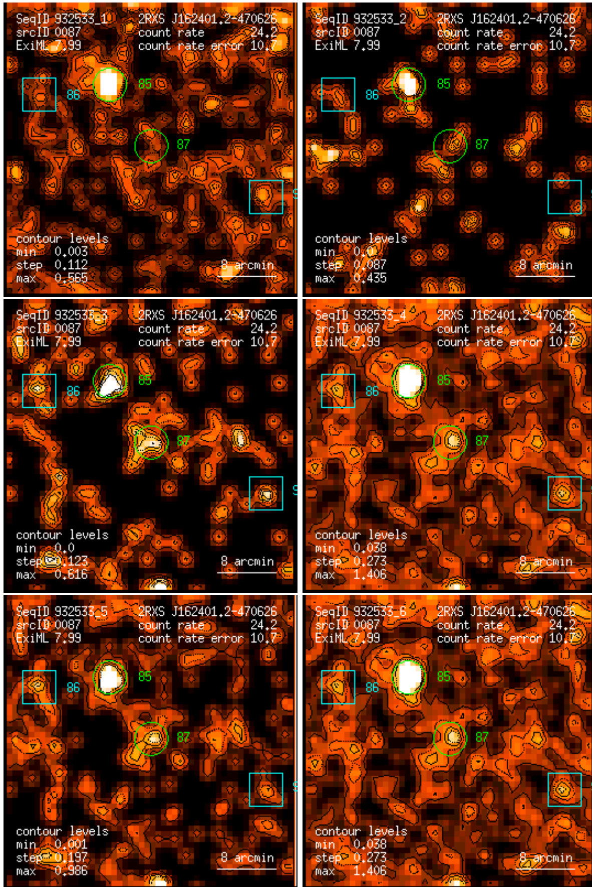
Figure 87: RASS 932533: detection 0087: band rate images, Gaussian filter: (1) PSPC channels 11 – 41, (2) 52 – 90, (3) 91 – 201, (4) 11 – 235, (5) 52 – 201, (6) 11 – 201. Broad band rates in counts/ks. Band rate contour levels in counts/ks/arcmin 2 .
